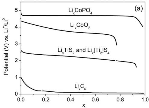
Figure 3. (a) Voltage profiles versus \text{Li}^+/\text{Li}^0 of the discharge curves of \text{Li}_x\text{C}_6 , \text{Li}_x\text{TiS}_2 and \text{Li}_x[\text{Ti}_2]\text{S}_4 , \text{Li}_x\text{CoO}_2 , and \text{Li}_x\text{CoPO}_4 . (b) Schematic of their corresponding energy vs density of states showing the relative positions of the Fermi energy in an itinerant electron band for \text{Li}_x\text{C}_6 , the \text{Ti}^{4+}/\text{Ti}^{3+} redox couple for \text{Li}_x\text{TiS}_2 and \text{Li}_x[\text{Ti}_2]\text{S}_4 , the \text{Co}^{4+}/\text{Co}^{3+} redox couple for \text{Li}_x\text{CoO}_2 , and the \text{Co}^{3+}/\text{Co}^{2+} redox couple for \text{Li}_x\text{CoPO}_4 . Reprinted with permission from Goodenough, J. B.; Kim, Y. Challenges for Rechargeable Li Batteries. Chem. Mater. 2010, 22 (3), 587–603. https://doi.org/10.1021/cm901452z . Copyright 2010 American Chemical Society.
