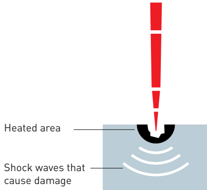
Nanosecond laser
