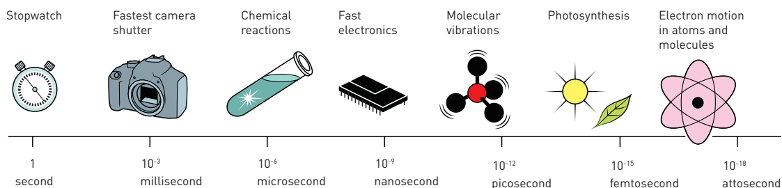
Figure 5. The faster the light pulses, the faster the movements that can be observed. The almost inconceivably short laser pulses are as fast as a few femtoseconds and can even be a thousand times faster, attoseconds. This allows sequences of events, which could once only be guessed at, to be filmed; the movement of electrons around an atomic nucleus can now be observed with an attosecond camera.
