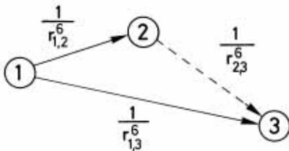
Figure 14. Spin diffusion. Transfer of magnetization between two hydrogen atoms 1 and 3 in the presence of additional hydrogen atoms goes through two competing pathways, i.e. , the direct NOE across the distance r_{1,3} , and two- or multiple-step spin diffusion via intervening hydrogen atoms.
