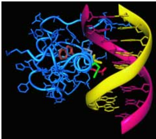
Figure 2. NMR structure of the complex formed between the Antennapedia homeodomain (blue, with functionally important residues in red, yellow, green and brown) and its operator DNA (yellow and red) (2).
