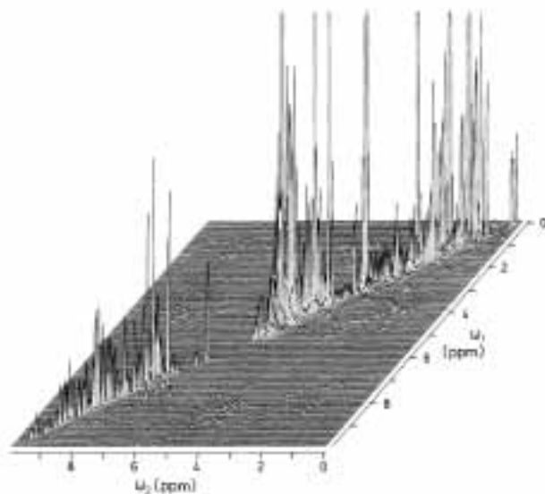
Figure 18. Two-dimensional (2D) [ ^1\text{H} , ^1\text{H} ]-NOE spectroscopy ([ ^1\text{H} , ^1\text{H} ]-NOESY). A stacked plot representation of a spectrum of the small protein bull seminal proteinase inhibitor IIA (BUSI IIA, M \approx 6000 ) is shown (500 MHz, 45°C, \text{H}_2\text{O} -solution).
