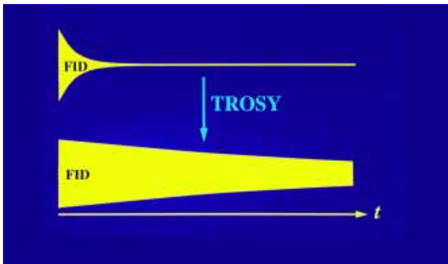
Figure 32. Schematic drawing of the free induction decay (FID) for a large protein with and without the use of TROSY. The period covered along the time axis is of the order of 100 milliseconds. The FID represents the primary recording of the NMR data in the “time domain”, from which the frequency domain spectrum (for example, Figures 18, 19 and 31) is obtained by Fourier transformation (31, 33).
