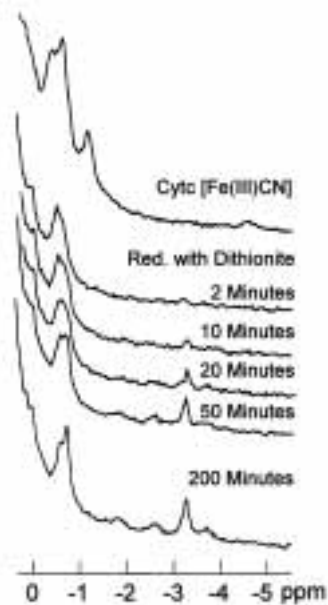
Figure 12. Changes with time in the 1D ^1\text{H} NMR spectrum of cytochrome c after reducing the ferric cyanide complex with dithionite (220 MHz, 9^\circ\text{C} , solvent ^2\text{H}_2\text{O} ).
