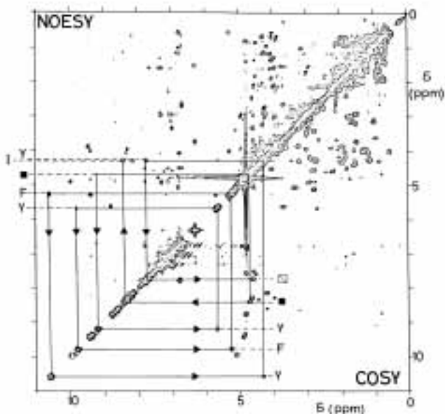
Figure 22. NOESY-COSY connectivity diagram for sequential ^1\text{H} NMR assignments using the d_{\alpha\text{N}} sequential NOEs. The data was recorded with BPTI in ^2\text{H}_2\text{O} solution. (see text).
