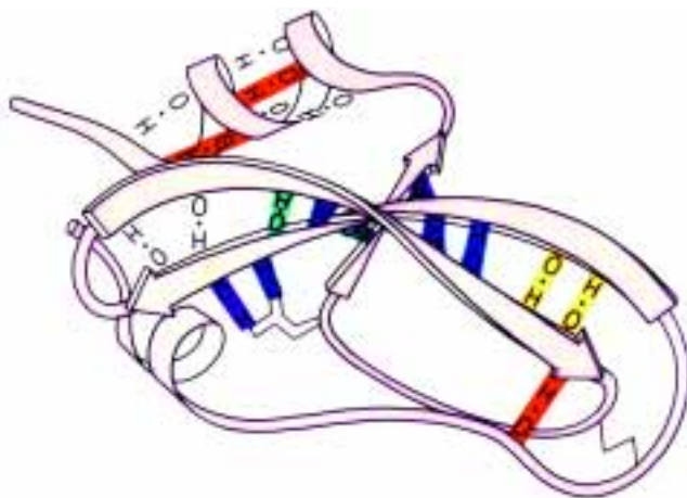
Figure 17. Sequence-specific resonance assignments for BPTI that were obtained using 1D ^1\text{H} NMR experiments (30). The polypeptide backbone is shown, and the assigned residues are identified by indication of hydrogen bonds with their amide protons (the colour code indicates variable exchange rates of the amide protons with the solvent; drawing by Jane Richardson, 1980).
