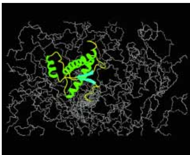
Figure 4. Visual impression of the variation of the bovine prion protein structure (Figure 3) during a time period of about 1 nanosecond. The superposition of 20 snapshots illustrates that the globular domain maintains its mean geometry, whereas the tail undergoes large-scale changes with time.
