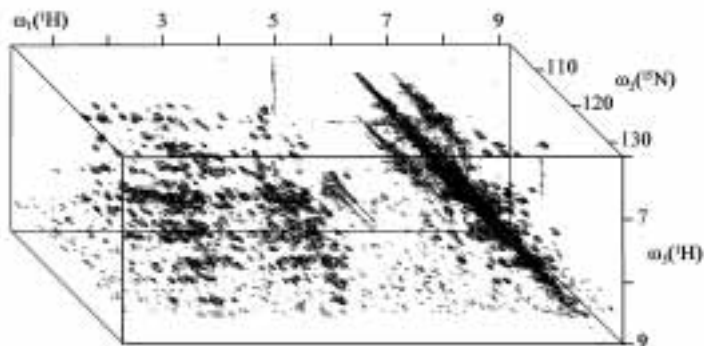
Figure 26. Three-dimensional (3D) ^{15}\text{N} -resolved [^1\text{H}, ^1\text{H}] -NOESY spectrum (600 MHz, 28^\circ\text{C} , \text{H}_2\text{O} -solution) of the DNA-binding domain of the P22 c2 repressor ( M \approx 10000 , uniformly ^{15}\text{N} -labeled).
