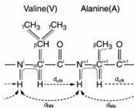
Figure 16. Sequential ^1\text{H} NMR assignment of proteins. The drawing shows the chemical structure of a -valine-alanine- dipeptide segment in a polypeptide chain. The dotted lines connect groups of hydrogen atoms that are separated by at most three chemical bonds and can therefore be connected using scalar spin-spin couplings. The broken arrows link neighbouring amino acid residues that are separated by short through-space distances, d_{\alpha\text{N}} and d_{\text{NN}} , and can therefore be connected by "sequential NOEs".
