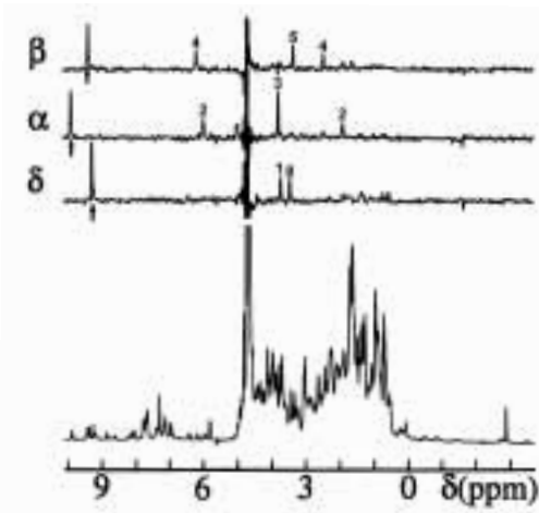
Figure 15. ^1\text{H} NMR assignments for the heme group of a c-type cytochrome using ^1\text{H} - ^{13}\text{N} NOEs (see Figure 7). Bottom trace: 1D ^1\text{H} NMR spectrum of ferrocyclochrome c-551 from Pseudomonas aeruginosa ( M \approx 12000 ). Upper traces: three 1D truncated-driven NOE difference spectra obtained with selective pre-irradiation (indicated by arrows) on the hydrogen atoms \beta , \alpha and \delta (see Figure 9), respectively (360 MHz, 35^\circ\text{C} , ^2\text{H}_2\text{O} -solution). The NOE peaks are identified with numbers indicating the substituents attached to the corresponding porphyrin ring carbons (Figure 9).
