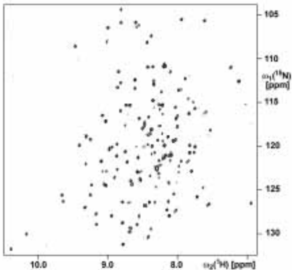
Figure 31. Transverse relaxation-optimized [ ^{15}\text{N} , ^1\text{H} ]-correlation spectroscopy (TROSY). A spectrum of the uniformly ^2\text{H} - and ^{15}\text{N} -labeled membrane protein OmpX reconstituted in DHPC micelles is shown (750 MHz, 30°C, \text{H}_2\text{O} -solution).
