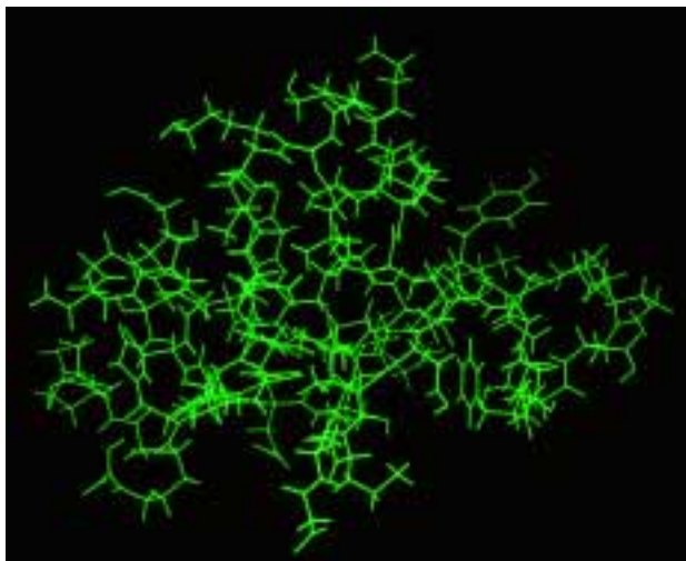
Figure 25. NMR structure of BUSI IIA (43).
