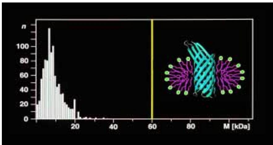
Figure 30. NMR structure determination and molecular weight. The horizontal axis covers the molecular weight-range 0 – 110'000. The left side shows the molecular weight distribution of the NMR structures in the protein databank (December 2000). On the right, the structure of the protein OmpX from E. coli ( M \approx 18000 ) in DHPC micelles ( M \approx 70\ 000 for the mixed micelles) indicates along the horizontal axis the approximate molecular weight range for NMR structure determination of mixed micelles with membrane proteins that is presently accessible with the NMR techniques of Figures 31 – 33.
