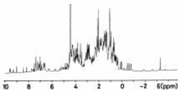
Figure 10. 1D ^1\text{H} NMR spectrum (360 MHz, 52^\circ\text{C} , solvent ^2\text{H}_2\text{O} ) of horse ferrocyanochrome c ( M \approx 12000 ).
