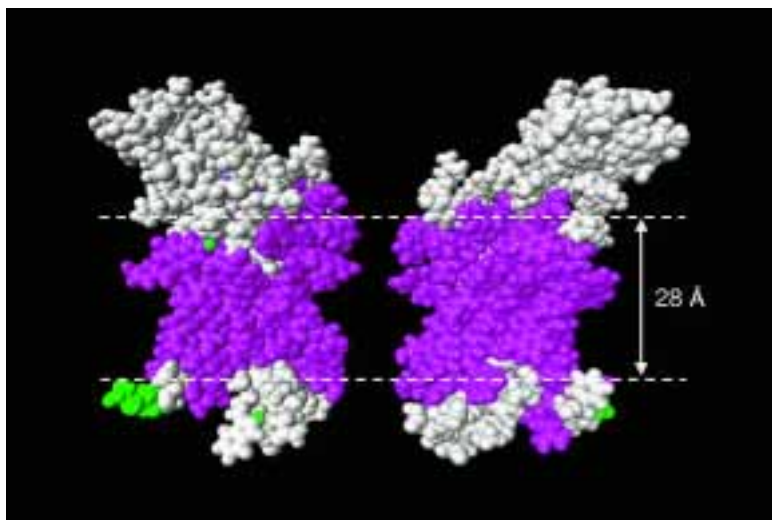
Figure 35. NMR structure of the membrane protein OmpX reconstituted in DHPC micelles. Front and back views of a space-filling model of OmpX are shown, with pink and green coloring identifying the surface area of the protein that is in contact with DHPC molecules in the mixed micelles. The two broken horizontal lines indicate the thickness of the lipid phase in the E. coli cell membrane.
