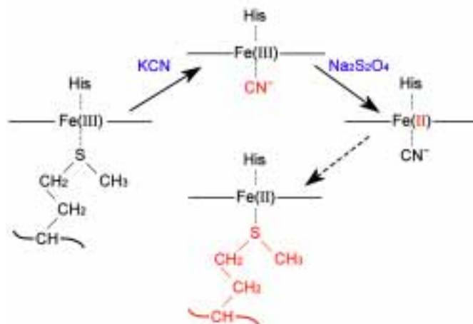
Figure 11. Three chemical reaction steps with cytochrome c that were used to identify methionine as one of the axial ligands of the heme iron (13). The roman numerals indicate the oxidation state of the heme iron, and His stands for the amino acid residue histidine. The solid and broken arrows indicate rapid and slow reaction steps, respectively. Colour code: black, heme iron with ligands, where the horizontal line through Fe represents a side view of the heme c ring (Figure 9); blue, chemicals added to the protein solution; red, new structural features resulting from the preceding reaction.
