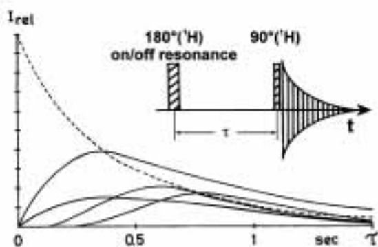
Figure 13. NOE build-up curves observed with 1D transient [ ^1\text{H}, ^1\text{H} ]-NOE measurements (26). The relative intensities, I_{\text{rel}} , of the pre-irradiated resonance line (broken curve) and of the lines experiencing NOEs (solid curves) are plotted versus the duration of the mixing period, \tau . The experimental scheme used to record transient NOE spectra (inset in the upper right) includes a selective 180^\circ radio-frequency pulse applied to the “pre-irradiated” ^1\text{H} NMR line, and a non-selective 90^\circ -pulse applied to the entire ^1\text{H} NMR spectrum. The two pulses are separated by the mixing period, \tau , and followed by signal acquisition. When working with the crowded spectra of proteins, one records the difference between two spectra obtained with the pre-irradiation 180^\circ(^1\text{H}) -pulse applied on- and off-resonance, respectively.
