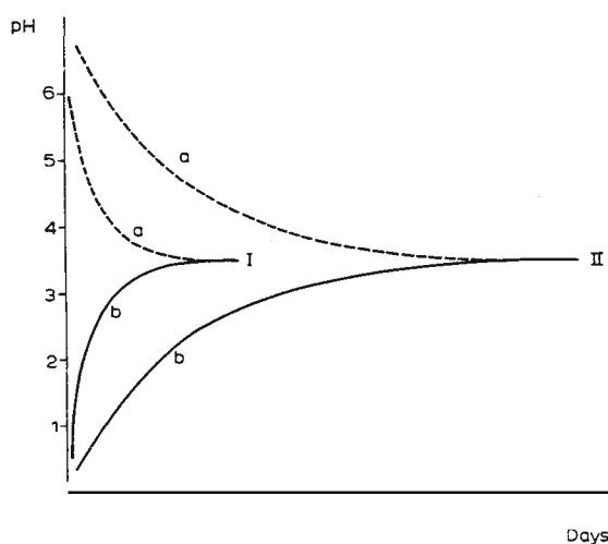
Fig. 4. Diagrammatic representation of equalization of acidity differences in fresh fodder to which sufficient acid has been added to reduce the fodder pH to 3-4. Curves a: pH changes in the solid phase of the fodder. Curves b: pH changes in the liquid phase of the fodder. I: Tests with chopped fodder. II: Tests with unchopped fodder.
