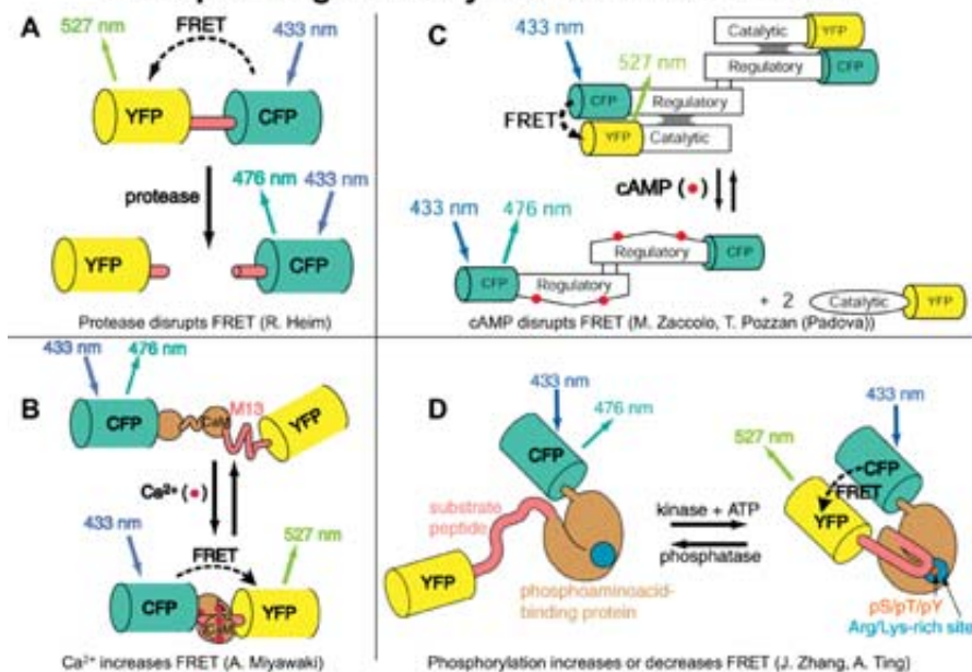
Figure 7. Schematic cartoons of genetically encoded fluorescent indicators based on FRET from CFP to YFP, to report A) protease activity, B) Ca 2+ concentrations, C) cAMP concentrations, and D) the balance between protein kinase and phosphatase activity.
