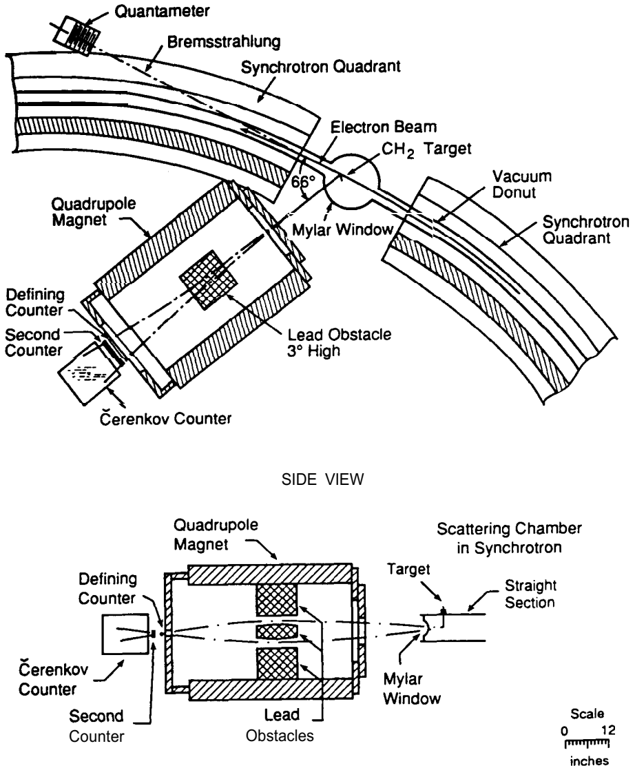
Fig. 24. Schematic of the equipment for electron scattering experiments at Cornell around 1960. These experiments used a quadrupole spectrometer to analyze electrons scattered from an internal target in the electron synchrotron. The target is mounted away from the normal orbit in the accelerator, and the beam is slowly moved onto the target after acceleration.
