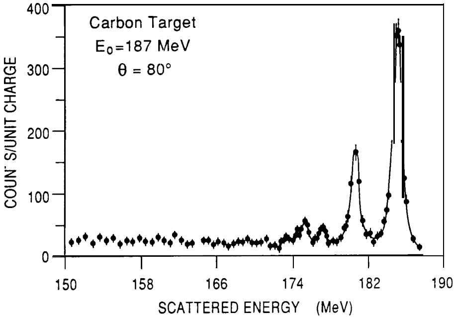
Fig. 3. Energy spectrum of 187 MeV electrons scattered through 80° by a carbon target, using the apparatus in Figure 2.
