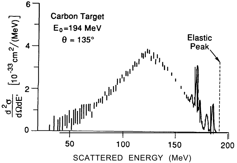
Fig. 30. Spectrum of electrons scattered inelastically from carbon. The excitation of nuclear levels is evident. The large, broad peak between 100 and 150 MeV is due to quasi-elastic scattering from the individual neutrons and protons that make up the carbon nucleus.
