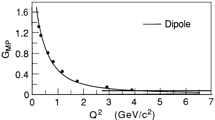
Fig. 25. G_M for the proton from data taken at CEA. The curve labelled "dipole" is a fit which originated in the late 1950's when the maximum measured Q^2 was limited to less than 1 \text{GeV}^2 . It has the form G_M = \mu_p / (1 + Q^2 / .71 \text{ GeV}^2)^2 and is in qualitative agreement with the CEA data at higher Q^2 , though the fit is not very good in the statistical sense.
