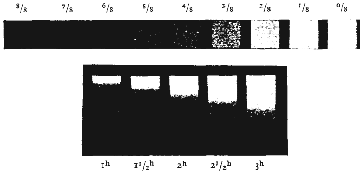
Fig. 10. Centrifugation of a solution of the compound of carbon monoxide and haemoglobin in a field of force 94,000 times gravity; time between exposures \frac{1}{2} hour; concentration scale at top.
