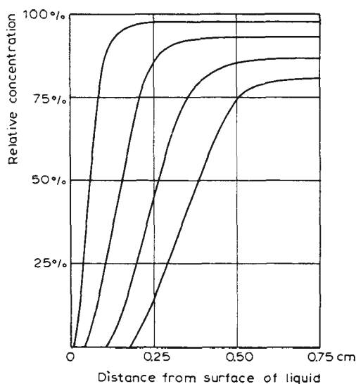
Fig. 6. Concentration distribution in a highly disperse gold colloid 5, 10, 15, 20 minutes after beginning of centrifugation; field of force 28,800 times gravity (according to H. Rinde).
