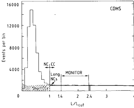
Figure 9 Identification, by the CDHS Collaboration, of NC events by their short event length. The peak at small event lengths is due to NC events. The long tail is due to muonic events, which must be subtracted under the peak to give the NC rate (Ref. 3).
