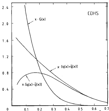
Figure 19 The gluon distribution G(x) derived from the QCD fits to F_L(x, Q^2) , \bar{q}(x, Q^2) , and xF_3(x, Q^2) (Ref. 10).
