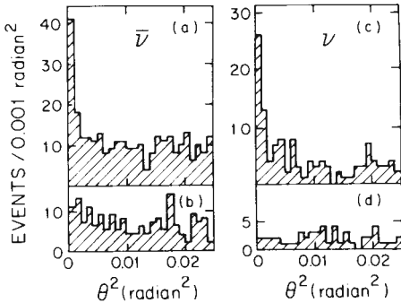
Figure 11 Identification of neutrino-electron events on the basis of their small angle with respect to the beam in the experiment of Ahrens et al. The peak at small angles in the two top graphs is due to neutrino-electron scattering. The bottom graphs show the flat distribution observed if photons rather than electrons are detected. This shows the angular distribution of background events.
