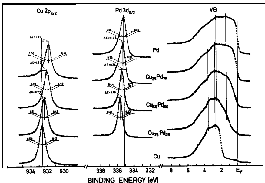
Fig. 5. Core and valence electron spectra (excited by monochromatized \text{AlK}\alpha -radiation) of some \text{Cu}_x\text{Pd}_{1-x} alloys, including the pure constituents. The binding energies undergo positive chemical shifts with increasing Cu-content. The asymmetries of the lines are due to creation of soft electron-hole pairs at the Fermi edge upon core ionization. The magnitude of the asymmetry is thus related to the (local) density of states at the Fermi level. The Pd lines are seen to become more symmetric as the Cu content increases (Pd local density of states decreases).
