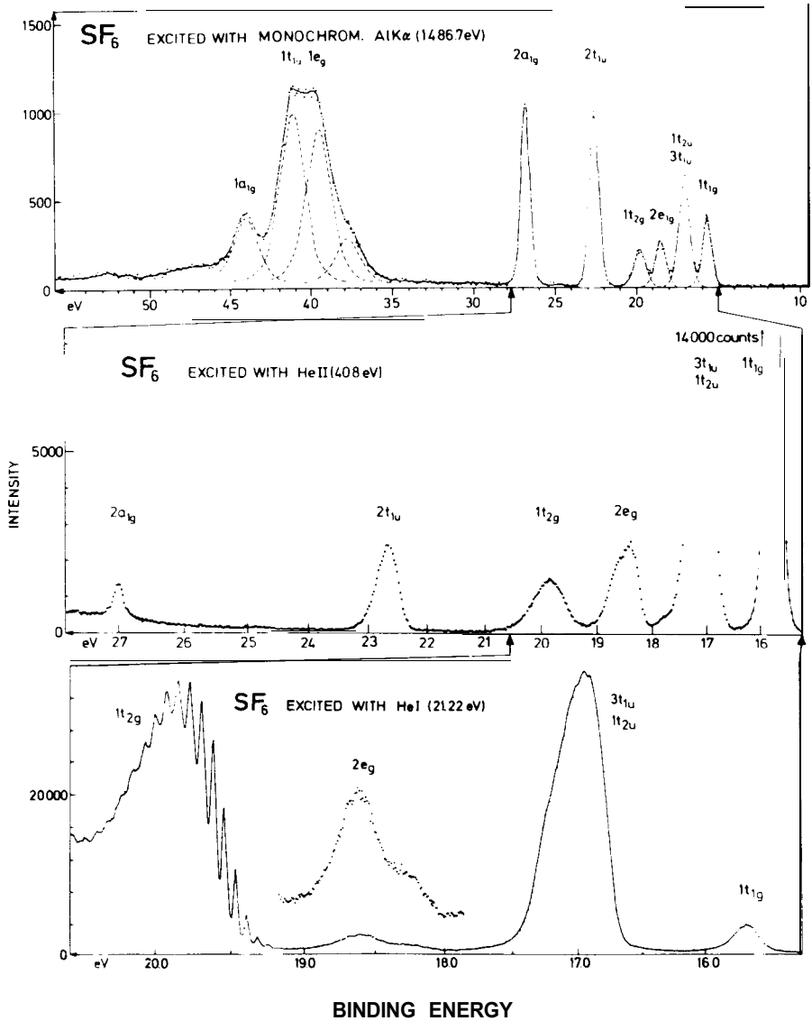
Fig. 14. Valence electron spectra of the \text{SF}_6 molecule excited with different photon energies ( \text{AlK}\alpha -, \text{HeII} and \text{HeI} -radiations). This figure illustrates the complementary nature of the various excitation sources. The \text{AlK}\alpha -excited spectrum enables a recording of the full valence region (including the innermost orbitals), which is not possible with the lower photon energies. The higher resolution in the spectra excited with the \text{He} resonance radiations allows the study of finer details of each of the outer electron bands. Note also the strong variations in the relative intensities of the bands as a function of photon energy. This can be used as an aid in assigning the spectrum / 197.198/.
