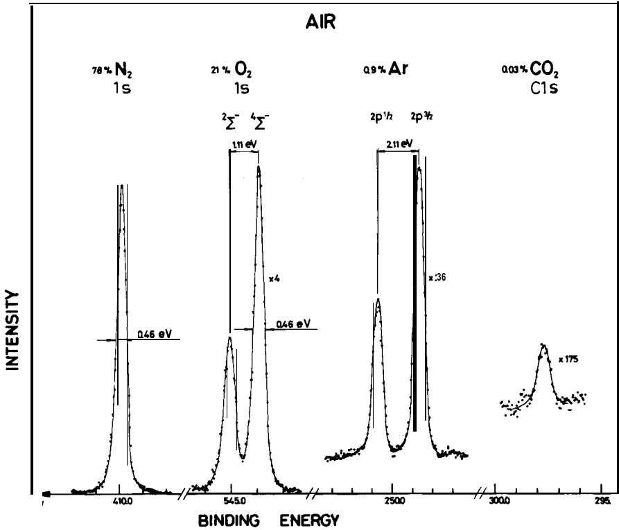
Fig. 9. Electron spectrum of air. The O_{1s} is split into two components due to 'spin' or 'multiplet' splitting. Excitation was performed by means of monochromatized AlK\alpha ( h\nu = 0.2eV ) radiation.
