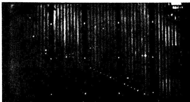
Figure 6. Some typical "vertex" events.
