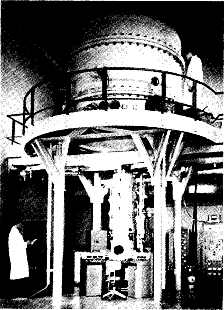
Fig. 17: 1 MV Electron Microscope (Japan Electron Optics Laboratory Co. Ltd.)
