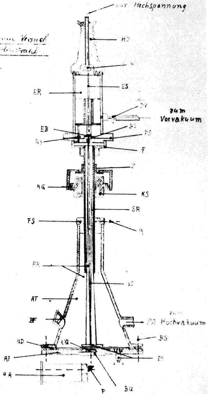
Fig. 1: Sketch by the author (1929) of the cathode ray tube for testing the imaging properties of the non-uniform magnetic field of a short coil [4. 5].
