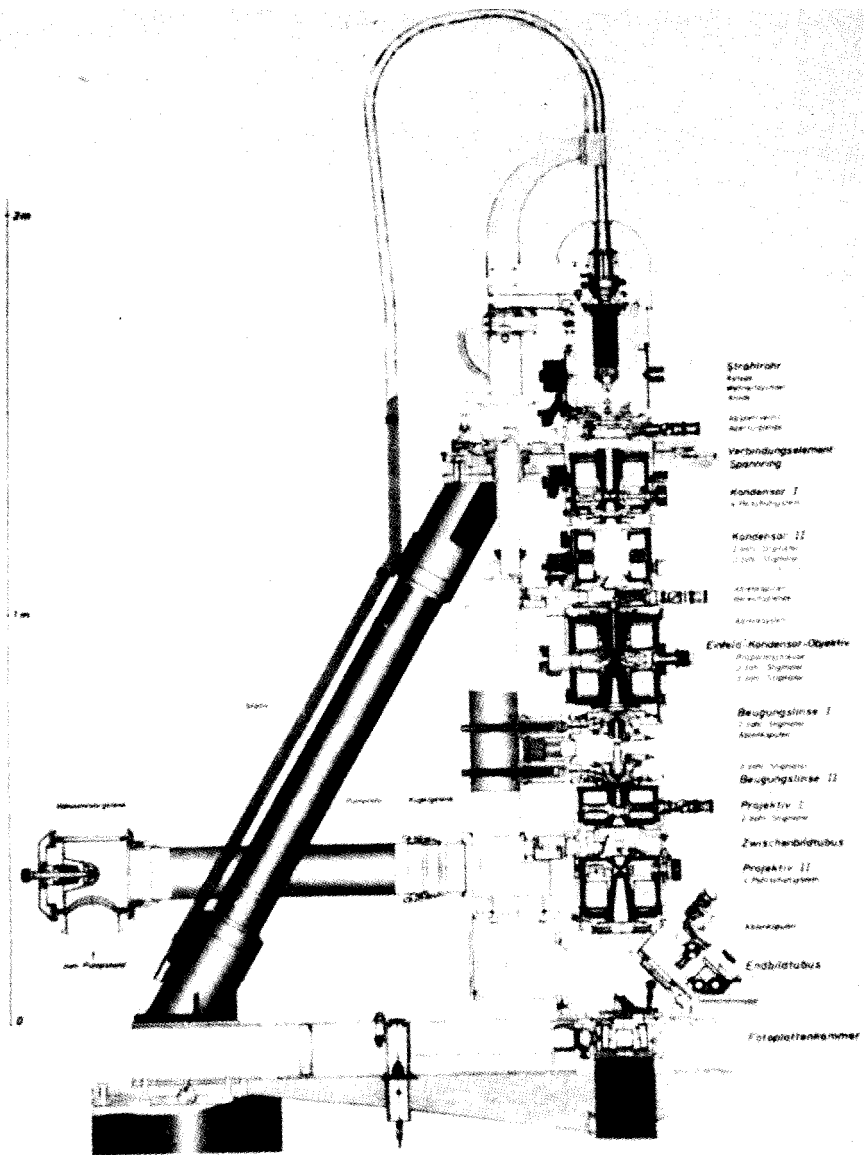
Fig. 14: Electron microscope with single-field condenser objective.
