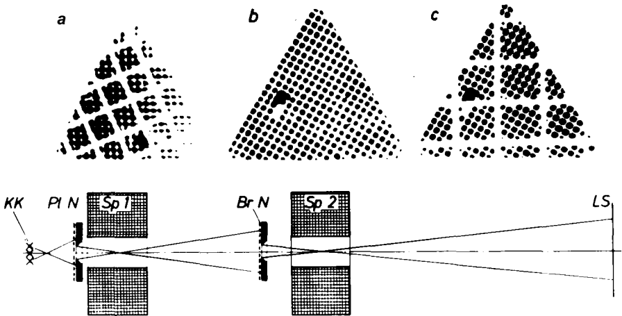
Fig. 3: First experimental proof (7 April 1931) that specimens (aperture grids) irradiated by electrons can be imaged in magnified form not only in one but also in more than one stage by means of (magnetic) electron lenses.
