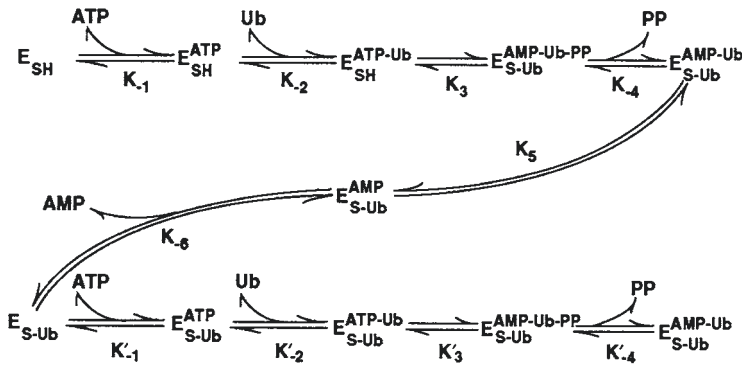
Scheme 1. The sequence and distribution of enzyme intermediates (Haas & Rose, 1982).
