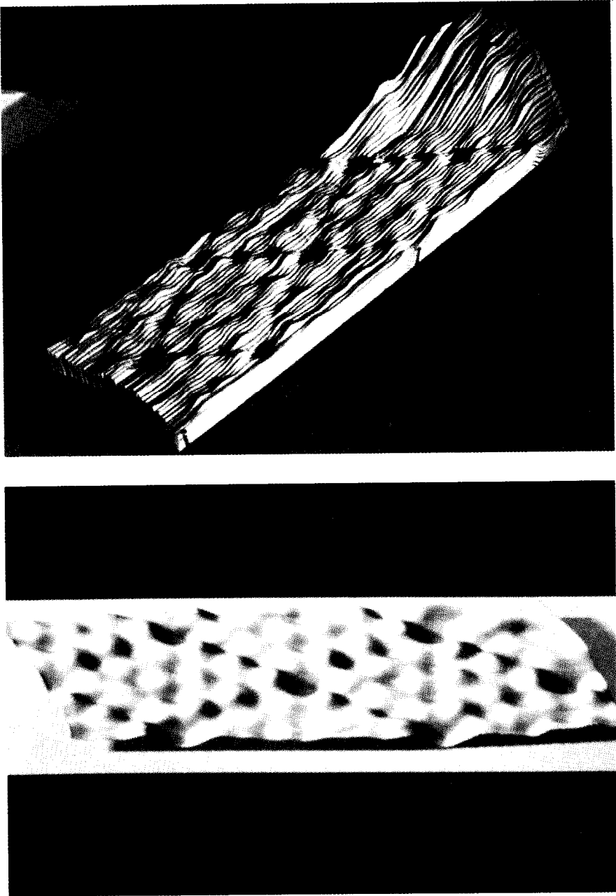
Fig. 6. 7 \times 7 reconstruction of Si(111), (a) Relief assembled from the original recorder traces, from Ref. [19], © 1983 The American Physical Society, and (b) processed image of the 7 \times 7 reconstruction of Si(111). Characteristic of the rhombohedral surface unit cell are the corner hole and the 12 maxima, the adatoms. In the processed image, the six adatoms in the right half of the rhombi appear higher. This is an electronic inequivalence on the surface owing to a structural left-right inequivalence in the underlying layers. The reconstruction extends undisturbed to the immediate vicinity of the large "atom hill" on the right.
