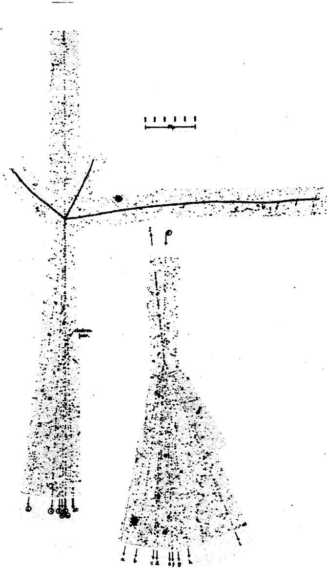
Fig. 7. A fast proton produces a disintegration (see the left-hand picture). One of the emerging «shower» particles (No. 5) after passing some millimeters in the emulsion, makes a second disintegration (see right-hand «star»).
