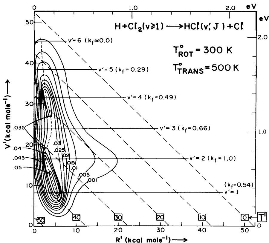
Figure 22. Effect of enhanced reagent internal energy on the product energy distribution, i. e., experimental k(V', R', T') , for \text{H} + \text{Cl}_2(v \geq 1) \rightarrow \text{HCl}(v', J) + \text{Cl} . This result is approximate since it was obtained by subtracting the detailed rate constants for \text{H} + \text{Cl}_2(v \approx 0) \rightarrow \text{HCl} + \text{Cl} from \text{H} + \text{Cl}_2(v \geq 0) \rightarrow \text{HCl} + \text{Cl} . Mean vibrational energy, \langle V \rangle \approx 3.3 kcal/mole. Compare with fig. 6. From A.M.G. Ding et al, Faraday Disc. Chem. Soc. 55, 252 (1973).
