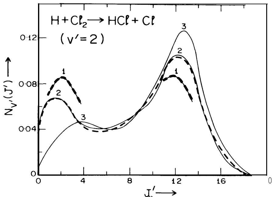
Figure 5. Solid lines record the decreasing contribution of the peak at low J' to the observed rotational distribution (for \text{H} + \text{Cl}_2 \rightarrow \text{HCl} + \text{Cl} (v' = 2, J') + \text{Cl} ) as the pressure in the beam-crossing region is decreased (in the sequence 3 \rightarrow 2 \rightarrow 1 ) in an A.R. vessel. The broken lines superimposed on the solid lines give relaxed distributions computed from 3. Based on fig. 1 of J.C. Polanyi and K.B. Woodall, J. Chem. Phys. 56, 1563 (1972).
