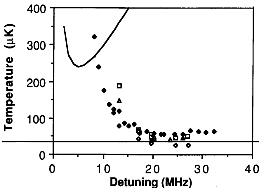
Figure 17. Dependence of molasses temperature on laser detuning (points) compared to the prediction of Doppler cooling theory (curve). The different symbols represent different molasses-to-probe separations.
