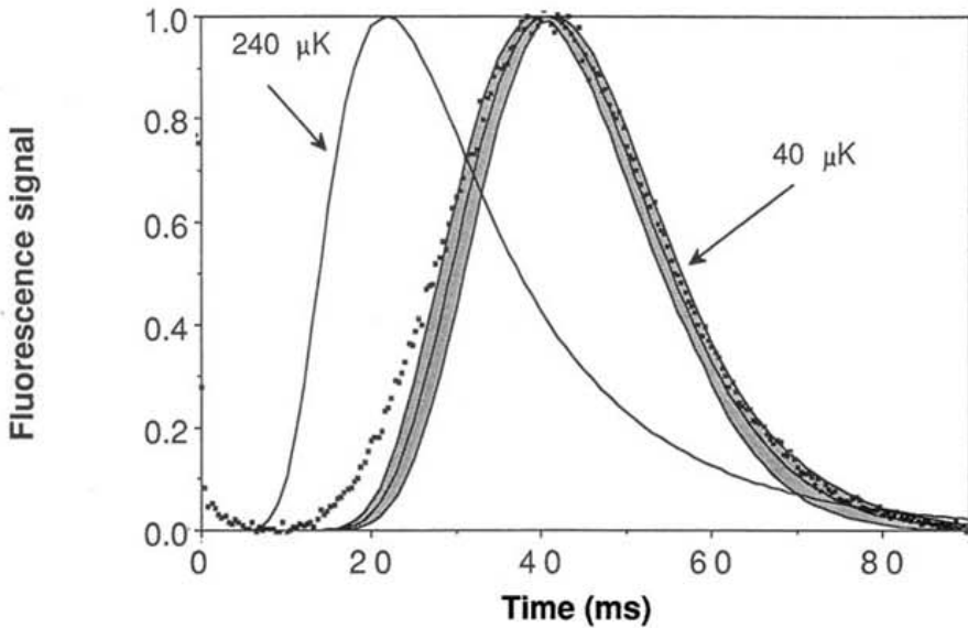
Figure. 16. The experimental TOF distribution (points) and the predicted distribution curves for 40\ \mu\text{K} and 240\ \mu\text{K} (the predicted lower limit of Doppler cooling). The band around the 40\ \mu\text{K} curve reflects the uncertainty in the measurement of the geometry of the molasses and probe.
