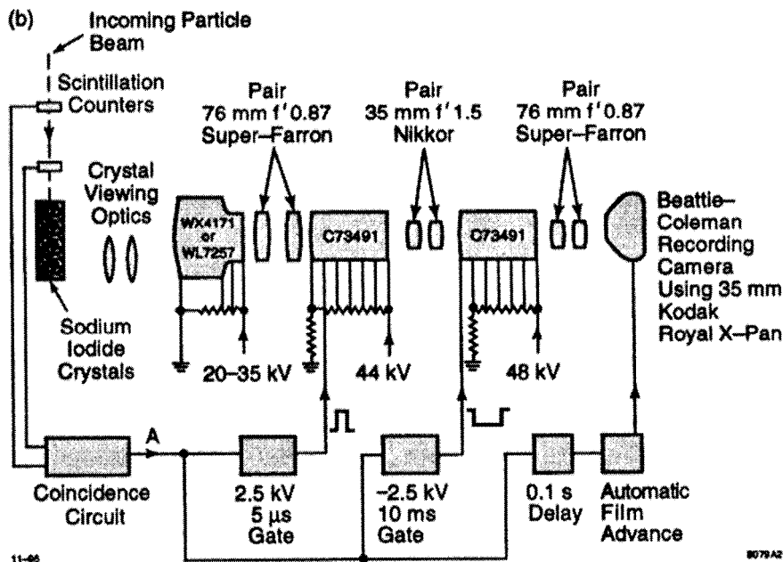
Figure 2. A novel track detector, the luminescent chamber, developed by Lawrence Jones and the author (Lai, Jones, and Perl, 1961) before the advent of the optical spark chamber. The caption read:
