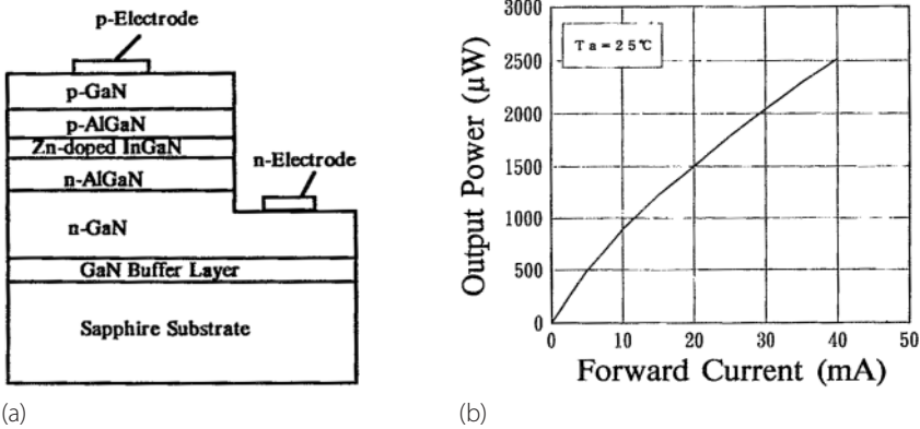
FIGURE 10. (a) Structure of InGaN/AlGaIn double-heterostructure blue LED with (b) resulting output power as a function of forward current. [23] (Reprinted with permission. Copyright 1994, AIP Publishing LLC.)
