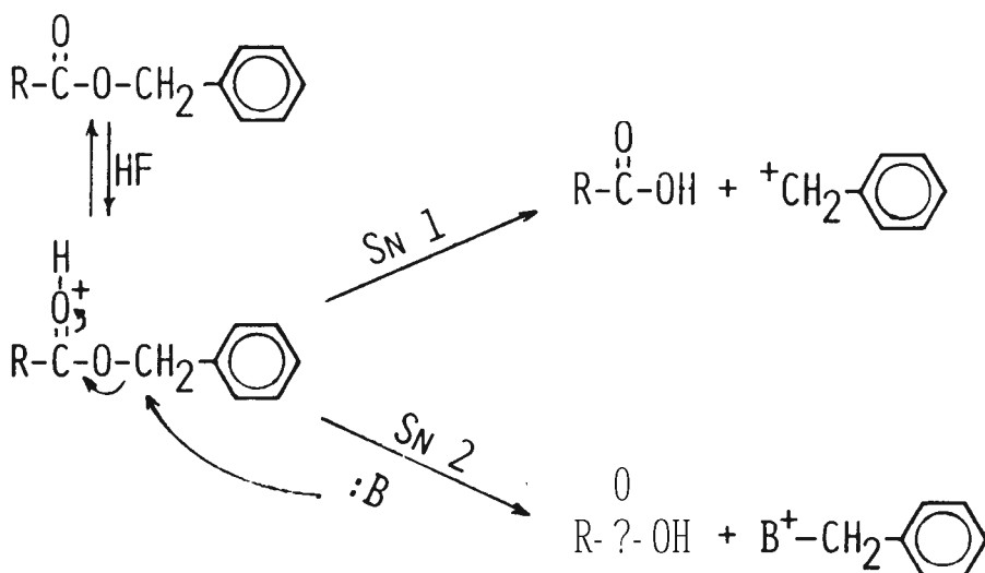
Fig. 14. The S_N1 and S_N2 acidolysis mechanisms.
