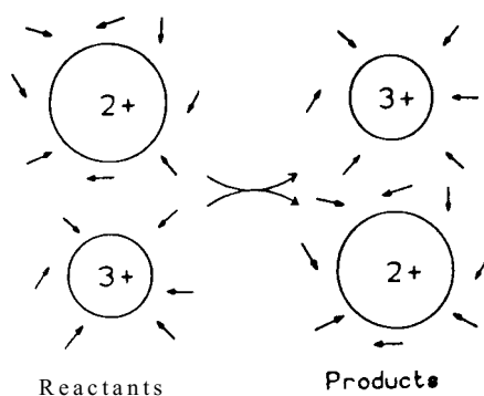
Figure 3. Typical nuclear configurations for reactants, products, and surrounding solvent molecules in reaction (1). The longer M-OH 2 bond length in the + 2 state is indicated schematically by the larger ionic radius. (Sutin, ref. 2)
