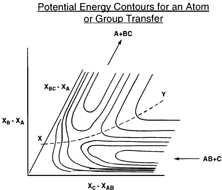
Figure 2. Potential energy contours for reaction (4), \text{AB} + \text{C} \rightarrow \text{A} + \text{BC} , in the collinear case.
