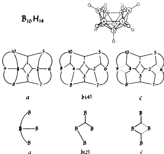
Fig. 30. The pattern of fractional bonds, dotted toward B 6 and B 9 , in B 10 H 14 can be expected when there is resonance of the type shown in the central diagram, or when one is tempted to draw open three-center BBB bonds as shown on the left. The fractional bond description is preferred.
