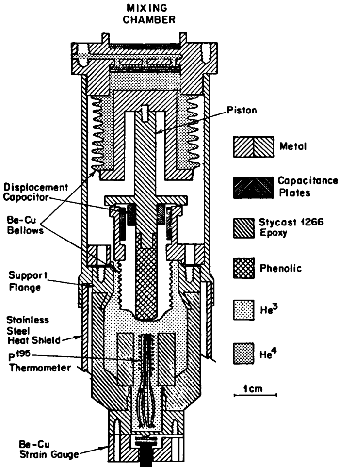
Figure 2. The Pomeranchuk cell used in the discovery experiments of Osheroff, Richardson and Lee. The pressure applied to the liquid {}^4\text{He} in the upper bellows causes a piston rod to drive the lower bellows into the {}^3\text{He} cell to increase the {}^3\text{He} pressure. The {}^4\text{He} bellows is larger than the {}^3\text{He} bellows, thus providing a favorable compression ratio, in analogy to a hydraulic press.
