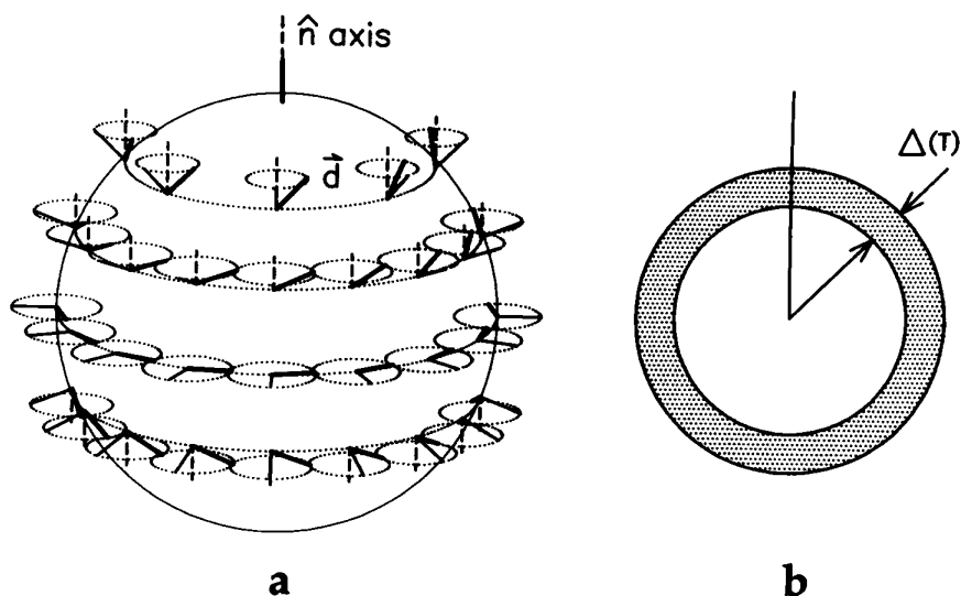
Figure 14. (a) The order parameter for superfluid {}^3\text{He B} showing \hat{d} vectors (represented by thick lines) rotated by 104^\circ about a vector \hat{n} from the radial directions (thin lines) for all points on the Fermi sphere. The rotation axis \hat{n} points in the vertical direction.
