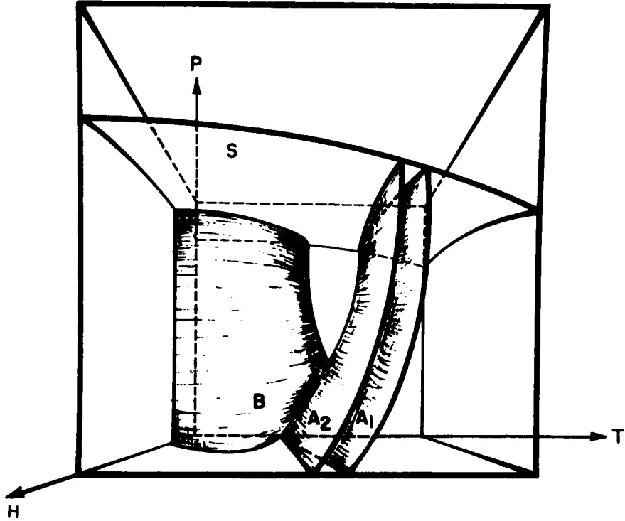
Figure 12. A schematic P-T-H diagram showing the general topology of the phase diagram of the superfluid phases, A, A_1 and B of liquid ^3\text{He} . The A_1 phase occurs between the surfaces labeled A_1 and A_2 . The A phase occurs at temperatures below the boundary labeled A_2 . The boundary between phases A and B is labelled B. The surface labelled S corresponds to the melting curve.
