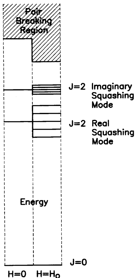
Figure 19. A schematic diagram showing the collective modes of superfluid {}^3\text{He B} discussed in the text. The left hand side of the diagram shows the zero field spectrum. The five fold degenerate j = 2 real squashing and imaginary squashing modes are shown as well as the pair breaking edge which is crudely analogous to the ionization energy of an atom. The right hand side of the diagram shows the five fold Zeeman splitting of these collective modes. The g factor of the imaginary squashing mode is smaller than that of the real squashing mode. The pair breaking edge occurs at a lower energy in a magnetic field partially as a result of gap distortion by the field.
