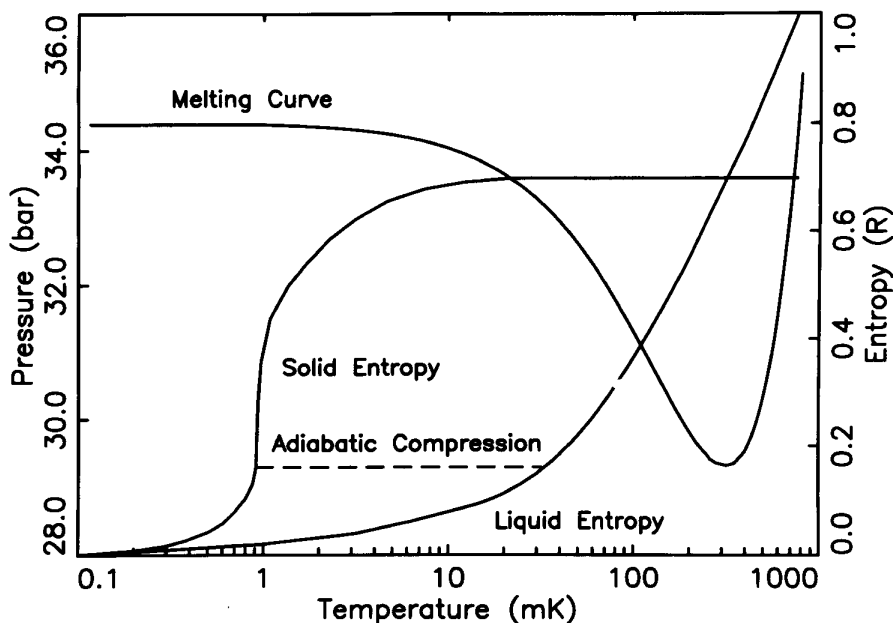
Figure 1. A semilog plot of the melting pressure of {}^3\text{He} versus temperature showing the minimum at 0.32 K and 29.3 bar. An idealized semilog plot of the entropy of liquid {}^3\text{He} and the entropy of solid {}^3\text{He} at the melting curve is shown on the same graph. For the highest temperatures, the liquid entropy was calculated from the melting curve via the Clausius Clapeyron equation and the assumption that S_{\text{solid}} = R \ln 2 . The two entropy curves cross at the melting curve minimum. The steep slope of the solid entropy curve near 1 mK corresponds to a magnetic phase transition in the solid. The dashed line is the path of an adiabatic compression from liquid to solid (Pomeranchuk cooling), to be discussed later.
