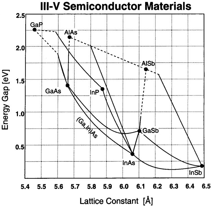
Figure 9. Partial “Map of the World,” plotting the energy gap of various III-V compounds vs. lattice constant. The map omits the “Old-World Continents” of the column-IV and the II-VI semiconductors, and the “New World” of the nitrides.
