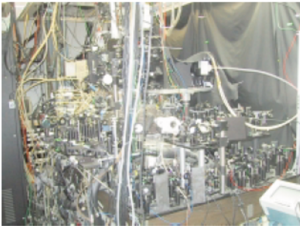
Figure 11. Comparison of a laser cooling and BEC experiment. The upper photograph shows the author in 1993 working on the Dark SPOT trap. In the following years, this laser cooling experiment was upgraded to a BEC experiment. The lower photograph shows the same apparatus in 2001 after many additional components have been added.
