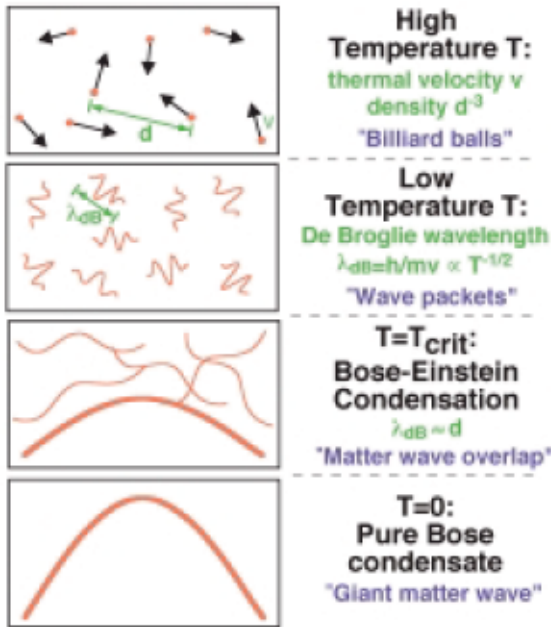
Figure 2. Criterion for Bose-Einstein condensation. At high temperatures, a weakly interacting gas can be treated as a system of “billiard balls.” In a simplified quantum description, the atoms can be regarded as wavepackets with an extension of their de Broglie wavelength \lambda_{dB} . At the BEC transition temperature, \lambda_{dB} becomes comparable to the distance between atoms, and a Bose condensate forms. As the temperature approaches zero, the thermal cloud disappears, leaving a pure Bose condensate.
