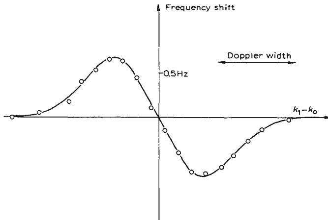
Fig. 15. Magnitude of shift as a function of k_1 - k_0 , k_0 , Center of optical absorption line of the atoms; k_1 center of acting radiation. k designates the wave number of the light. (Cohen-Tannoudji 51 )
