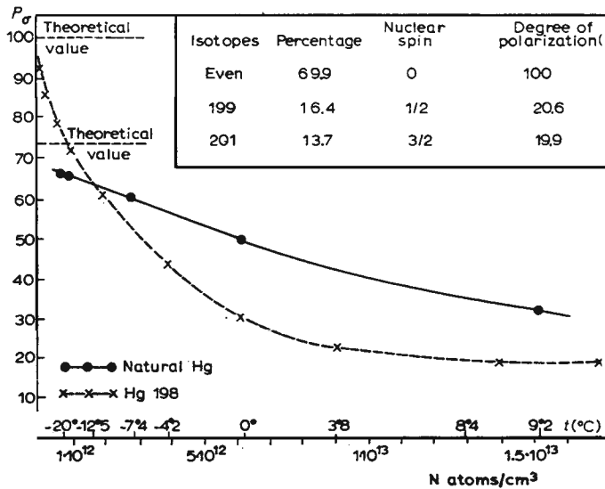
Fig. 2. Degree of polarization of optical resonance light at 2537 Å as a function of vapor density for natural mercury and for the pure ^{198}\text{Hg} isotope. (Rollet, Brossel and Kastler 26 )
