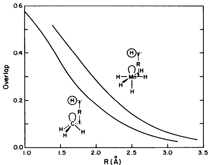
Figure 2. Overlap integrals between the a_1 frontier orbital of \text{MnH}_5^+ and \text{CH}_3 and a H 1s orbital at a distance R from the Mn or C.
