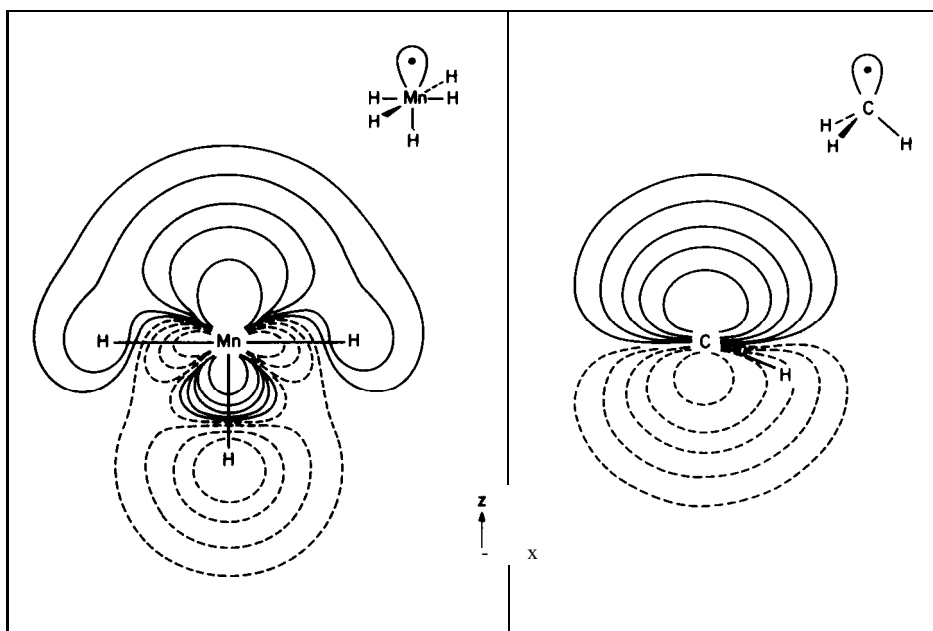
Figure 1. Contour diagram of the isolobal a_1 orbitals of \text{MnH}_5^{5-} (left) and \text{CH}_3 (right), as computed by the extended Hückel method. The contours of \psi , plotted in a plane passing through Mn and three H's (left) and C and one H (right), are \pm 0.2 , \pm 0.1 , \pm 0.55 , \pm 0.25 , \pm 0.1 .
