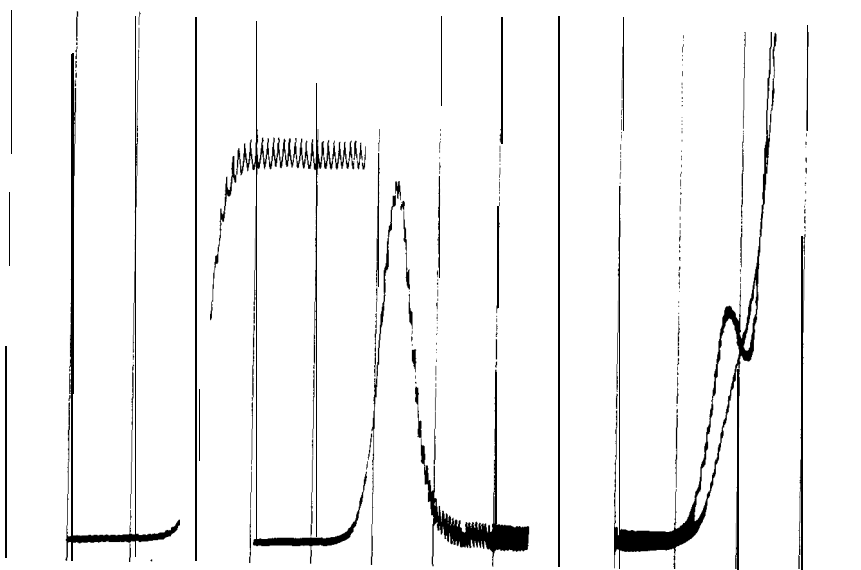
Fig. 17. Primitive and derivative polarographic curves: (left) 0.001 M CdCl 2 in ammonia buffer solution, 0.1 N NH 3 in NH 4 Cl; (right) 0.001 M CdCl 2 in 0.1 N LiOH.
