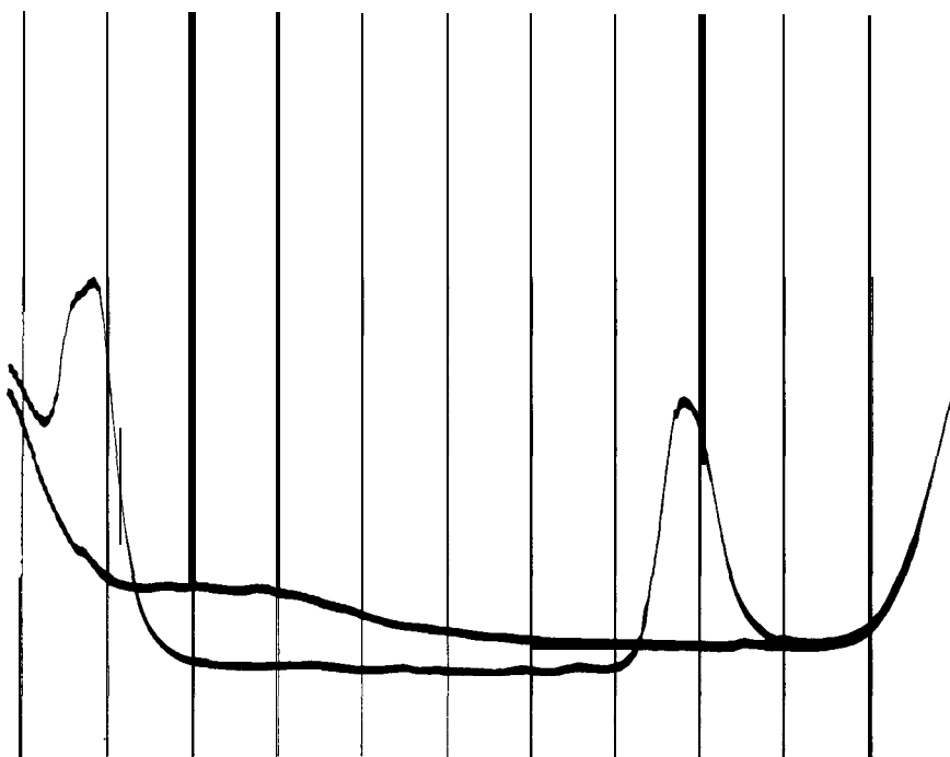
Fig. 24. Tensammetric maxima due to adsorption and desorption of cyclohexanol in acetate buffer solution. ( Upper curve : pure solution).
