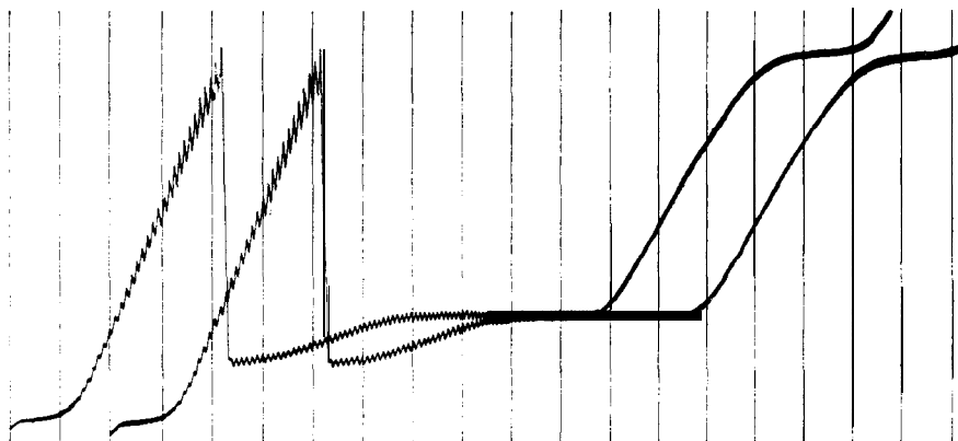
Fig. 14. Maximum of the first order on the wave of oxygen in 0.001 M KCl.
