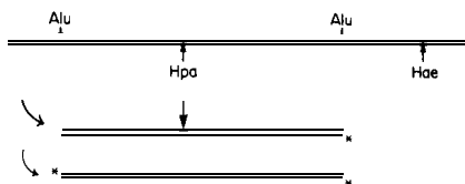
Figure 2. Procedure for obtaining a double-stranded DNA fragment uniquely labeled at one end of one strand. The figure shows the restriction cuts for the enzymes AluI (target AG/CT) and HpaI (target C/CGG producing an uneven end) in the neighborhood of the lac operator. The lac repressor is shown bound to the DNA. By cutting the DNA from this region first with the enzyme AluI , then labeling with radioactive P^{32} the 5' termini of both strands of the DNA with polynucleotide kinase, and then cutting in turn with the enzyme HpaI , we can isolate a DNA fragment that carries the binding site for the repressor uniquely labeled at one end of one strand.
