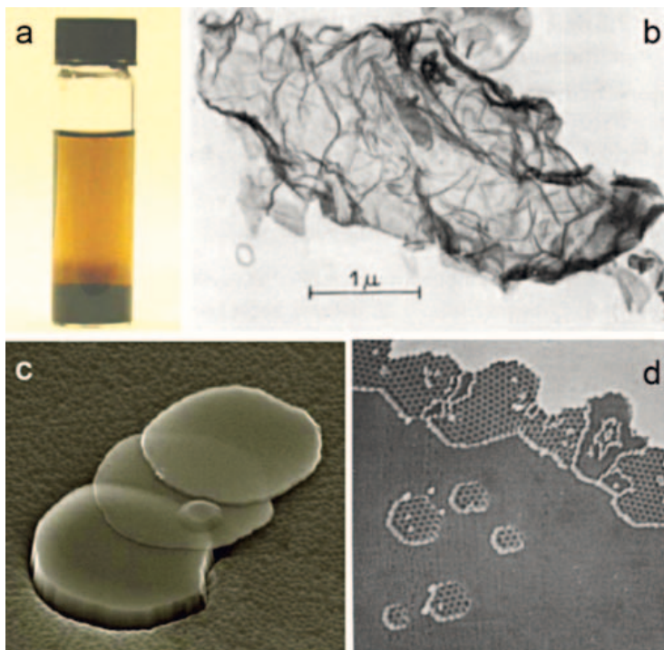
Figure 3. Prehistory of graphene. a – Graphene as probably seen by Brodie 150 years ago. Graphite oxide at the bottom of the container dissolves in water making the yellow suspension of floating graphenic flakes. b – TEM image of ultra-thin graphitic flakes from the early 1960s (copied with permission from ref. [43]). c – Scanning electron microscopy (SEM) image of thin graphite platelets produced by cleavage (similar to images reported in ref. [60]). d – STM of graphene grown on Pt (copied with permission from ref. [53]). The image is 100x100 nm 2 in size. The hexagonal superstructure has a period of ~22 Å and appears due to the interaction of graphene with the metal substrate.
