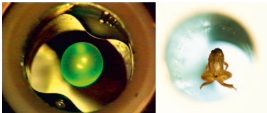
Figure 1. Levitating moments in Nijmegen. Left – Ball of water (about 5 cm in diameter) freely floats inside the vertical bore of an electromagnet. Right – The frog that learned to fly. This image continues to serve as a symbol showing that magnetism of 'nonmagnetic things', including humans, is not so negligible. This experiment earned Michael Berry and me the 2000 Ig Nobel Prize. We were asked first whether we dared to accept this prize, and I take pride in our sense of humour and self-deprecation that we did.
