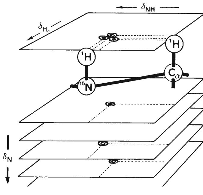
Figure 23. 3D resolution of a 2D proton-resonance spectrum by ^{15}\text{N} resonance spreading. The NH-C \alpha H cross peaks are displaced in a third dimension by the corresponding ^{15}\text{N} chemical shifts.
