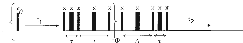
Figure 19. Pulse sequence for C_1 spin topology filtration consisting of \pi/2 and \pi pulses. The delays are adjusted to \tau = 1/(8J) and \Delta = 1/(2J) where J is the uniform J -coupling constant. \Phi is phase-cycled for four-quantum selection and \Theta for the suppression of axial peaks (94).
