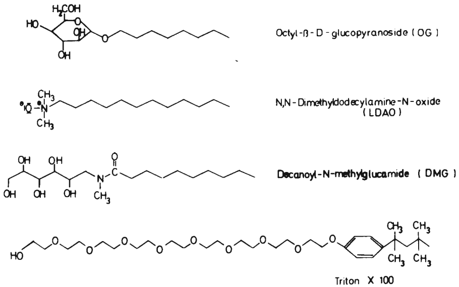
Figure 4: Structural formulas of commonly used detergents: octylglucopyranoside, N,N -dimethyldodecylamine- N -oxide, decanoyl- N -methylglucamide are promising for membrane protein crystallization, whereas Triton X100 is not.
