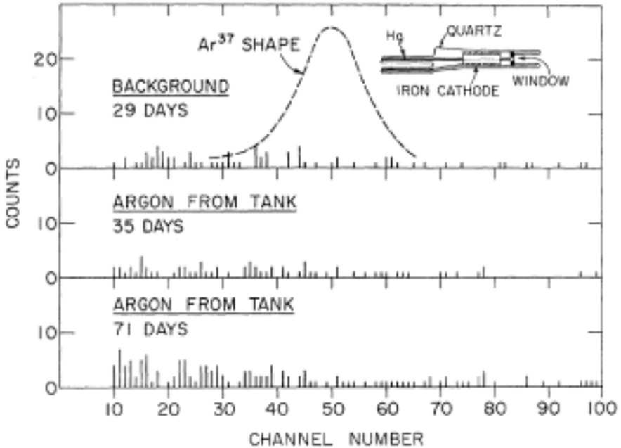
Figure 14. Pulse-height spectra from the first two runs on the chlorine experiment. No counts in excess of background were detected in either run. Figure from Davis et al. (1968).
