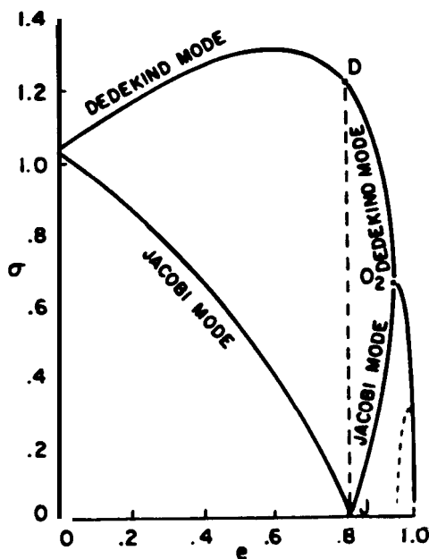
Fig. 7. The characteristic frequencies (in the unit (\pi G\rho)^{1/2} ) of the two even modes of second-harmonic oscillation of the Maclaurin spheroid. The Jacobi sequence bifurcates from the Maclaurin sequence by the mode that is neutral ( \sigma = 0 ) at e = 0.813 ; and the Dedekind sequence bifurcates by the alternative mode at D. At O_2 , ( e = 0.9529 ) the Maclaurin spheroid becomes dynamically unstable. The real and the imaginary parts of the frequency, beyond O_2 are shown by the full line and the dashed curves, respectively. Viscous dissipation induces instability in the branch of the Jacobi mode; and radiation-reaction induces instability in the branch DO_2 of the Dedekind mode.
