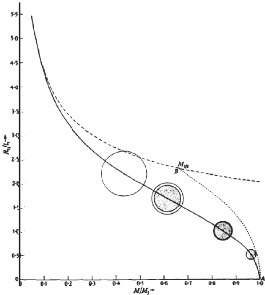
Fig. 2. The full-line curve represents the exact (mass-radius)-relation ( l_1 is defined in equation (46) and M_1 denotes the limiting mass). This curve tends asymptotically to the --- curve appropriate to the low-mass degenerate configurations, approximated by polytropes of index 3/2 . The regions of the configurations which may be considered as relativistic ( Q > (K_1/K_2)^3 ) are shown shaded. (From Chandrasekhar, S., Mon. Not. Roy. Astr. Soc. , 95, 207 (1935).)
