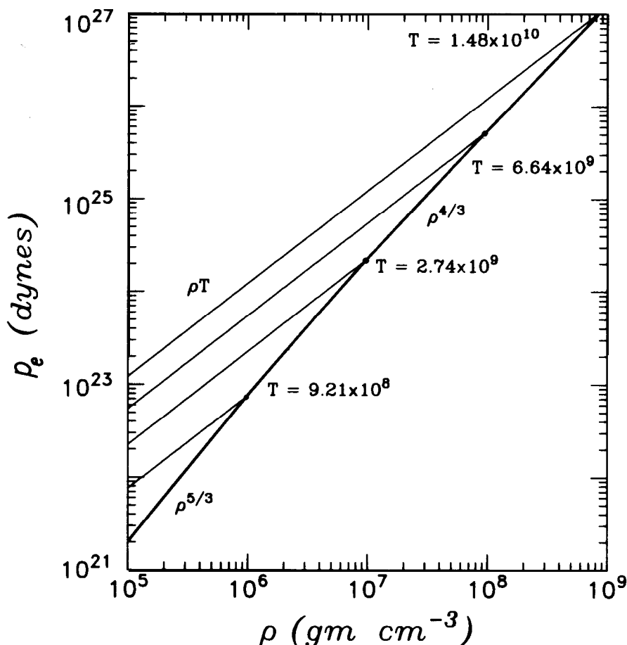
Fig. 4. Illustrating how by increasing the density at constant temperature degeneracy always sets in.
