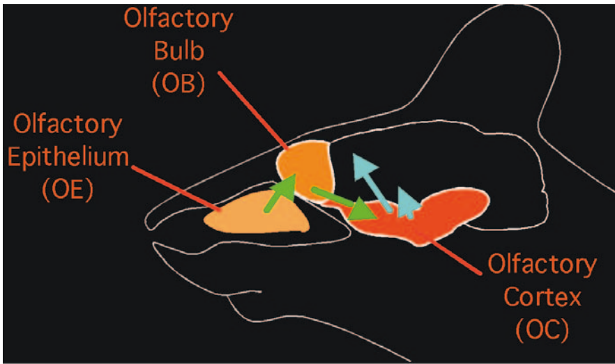
Figure 2. The olfactory pathway. Odorants are detected by olfactory sensory neurons in the olfactory epithelium. Signals generated in those neurons are relayed through the olfactory bulb to the olfactory cortex and then sent to other brain areas.
