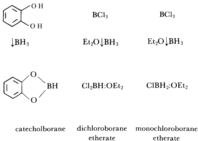
Fig. 6. The synthesis of heterosubstituted boranes
