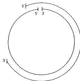
Fig. 3. Structure of the DNA extracted from Dane particles proposed by Summers et al. (26). The position of the gaps in the single strands, and the location of the 5' and 3' ends are shown.
