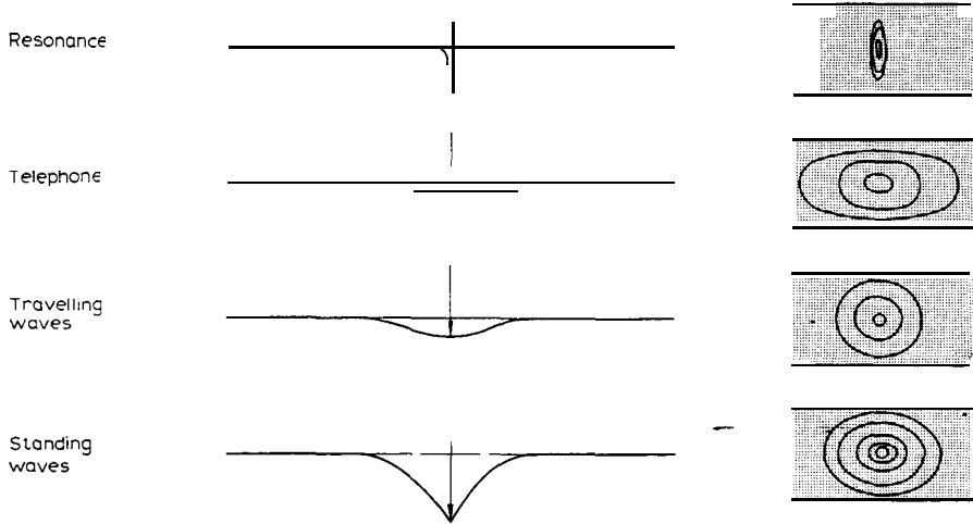
Fig. 21. Different types of deformation produced in a rubber membrane, depending on the thickness and the lateral stress of the membrane.
