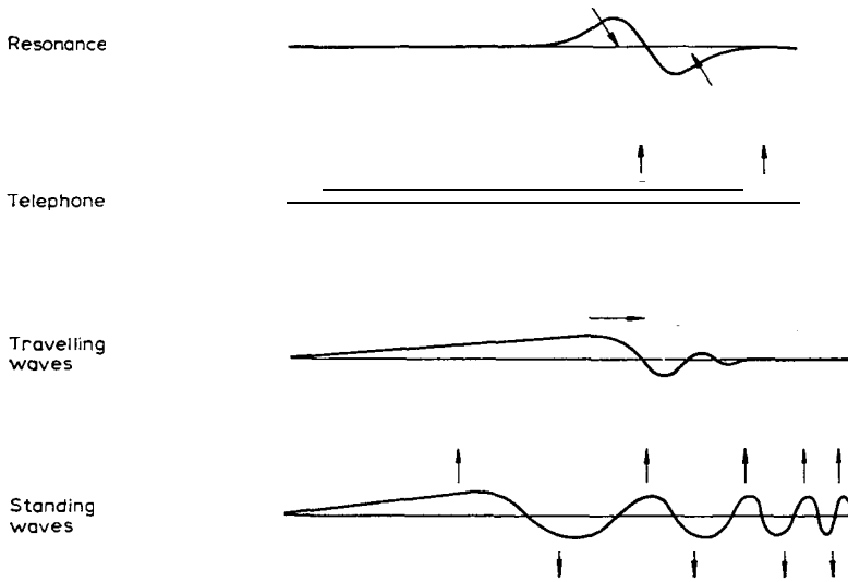
Fig. 22. All the different hearing theories form one family of vibration patterns, differing only in the stiffness of the membrane.
