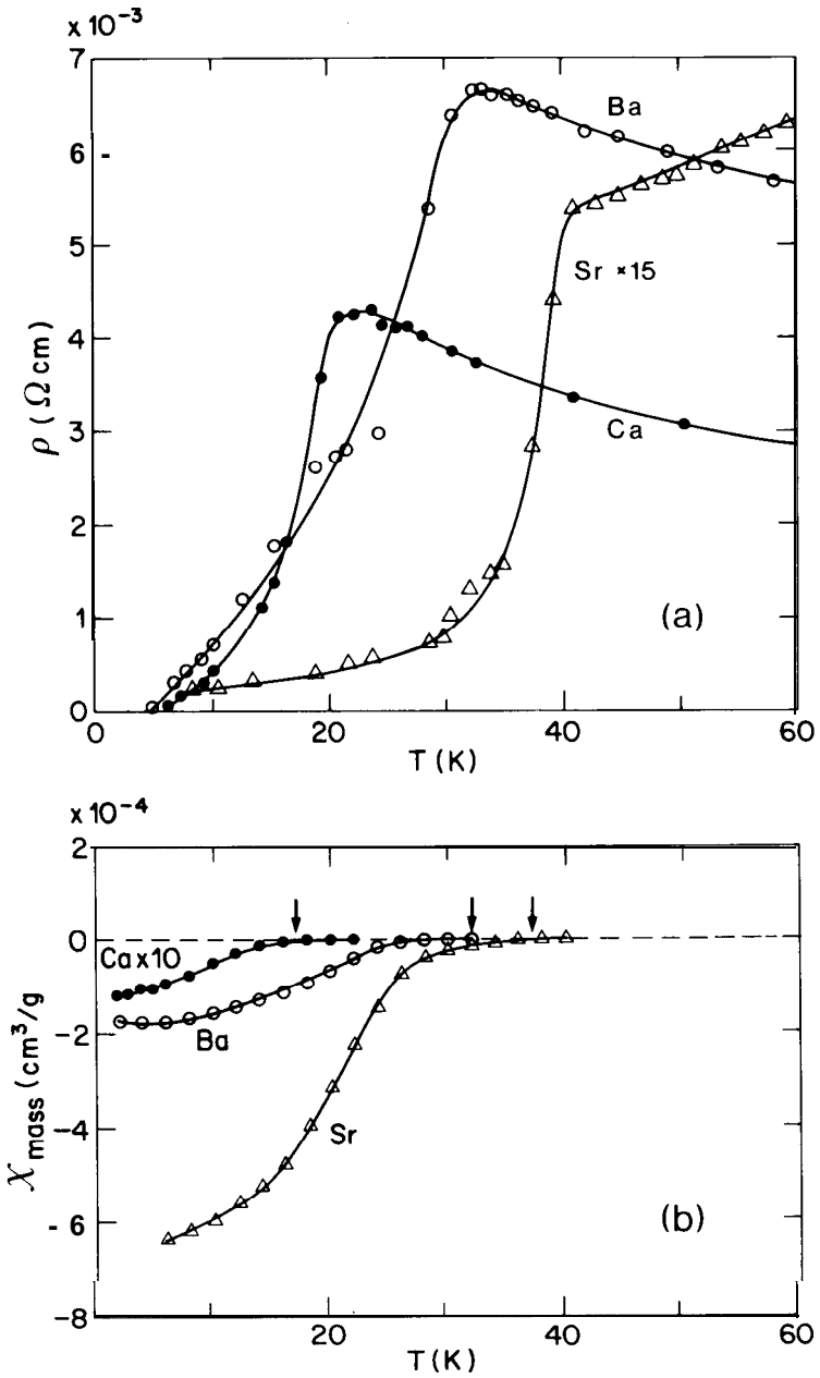
Figure 1.12. (a) Resistivity as a function of temperature for Ca ( \bullet ), Sr ( \Delta ), and Ba ( \circ ) substitution with substituent-to-La ratios of 0.2/1.8, # 0.2/1.8, 0.15/1.85, respectively. The Sr curve has been vertically expanded by a factor of 15. (b) Magnetic susceptibility of these samples. The substituents are Ca ( \bullet ), Sr ( \Delta ), and Ba ( \circ ), with total sample masses of 0.14, 0.21, and 0.13 g, respectively. The Ca curve has been expanded by a factor of 10. Arrows indicate onset temperatures. From [1.25], © 1987 by the American Association for the Advancement of Science.
