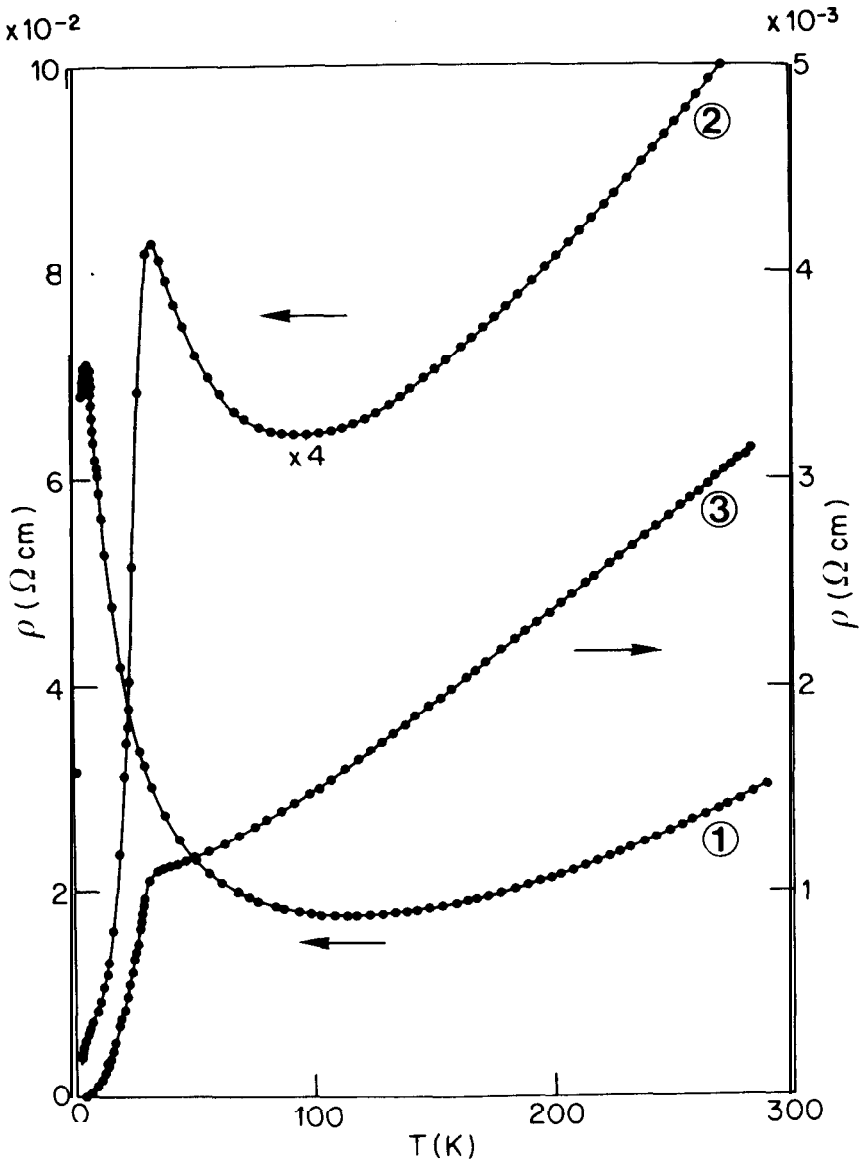
Figure 1.9. Resistivity as a function of temperature for \text{La}_2\text{CuO}_{4-x}:\text{Ba} samples with three different Ba:La ratios. Curves 1, 2, and 3 correspond to ratios of 0.03, 0.06, and 0.07, respectively. From [1.20], © 1987 Pergamon Journals Ltd.
