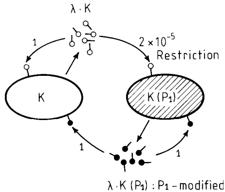
Fig 2: PI-specific restriction and modification as detected by growth of bacteriophage \lambda .
