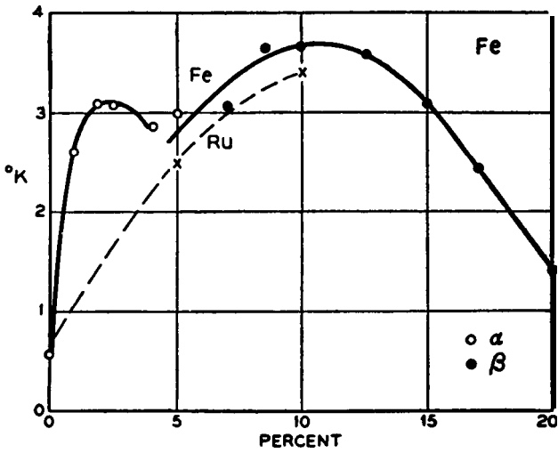
Superconducting transition temperatures of iron or ruthenium solid solutions in titanium.
