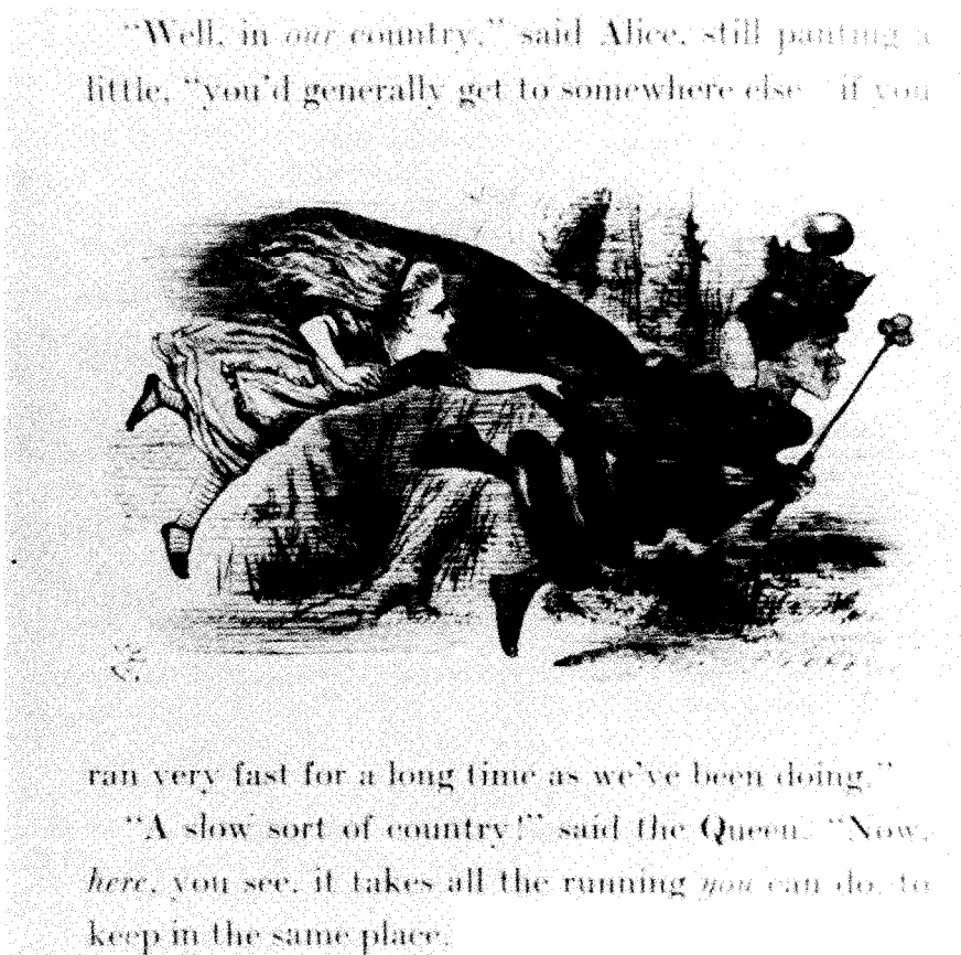
Fig. 19. Efforts to avoid localization (Dodson).
