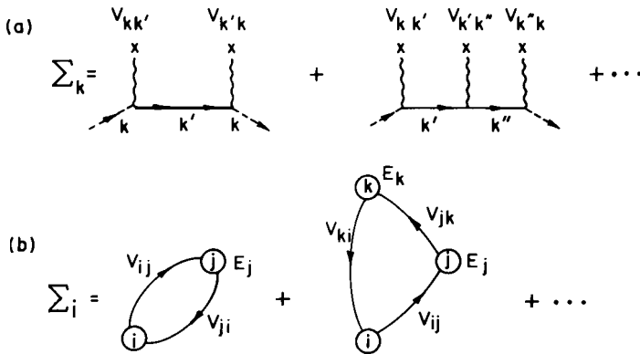
Fig. 15. a) Self-energy diagrams in conventional "propagator" theory. b) Self-energy diagrams in "locator" theory.
