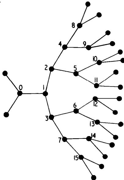
Fig. 17. "Cayley Tree" on which localization theory is exact.
