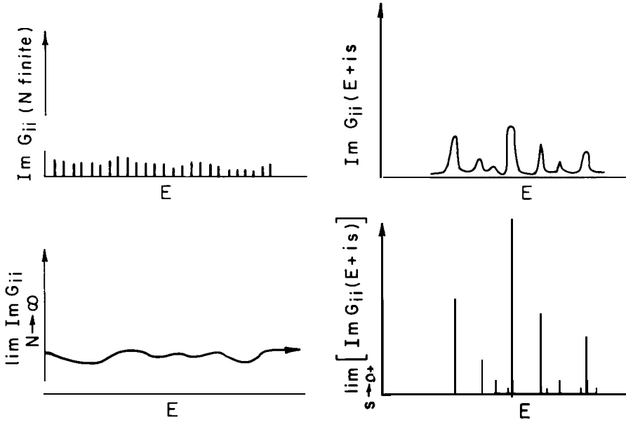
Fig. 16. a) \text{Im } G_{ii} in extended case b) \text{Im } G_{ii} in localized case
