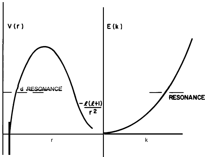
Fig. 4. d -Resonance due to tunneling through the centrifugal barrier.
