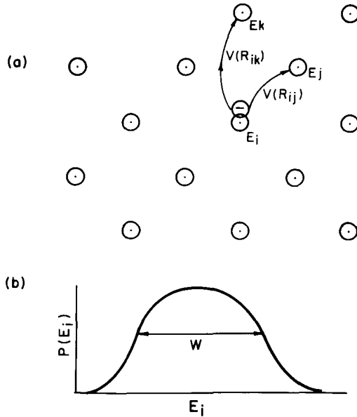
Fig. 14. Model for diffusion in a random lattice
