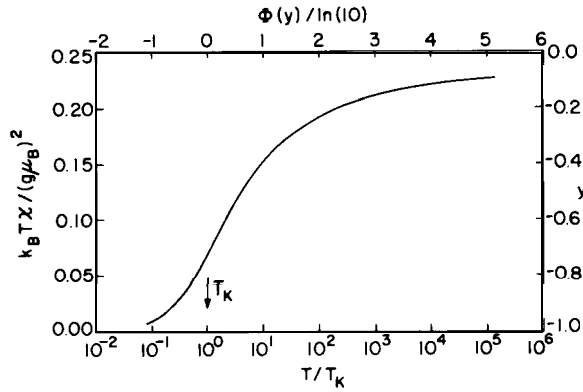
Fig. 7. Susceptibility of the Kondo Model as calculated by Wilson.
