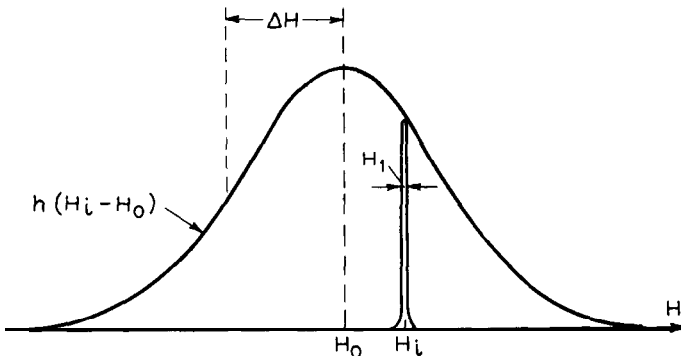
Fig. 13. “Spin packets” and spectral diffusion.
