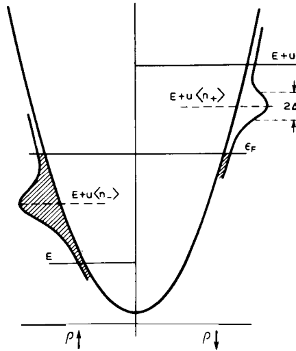
Fig. 5. Spin-split energy levels in the magnetic case.
