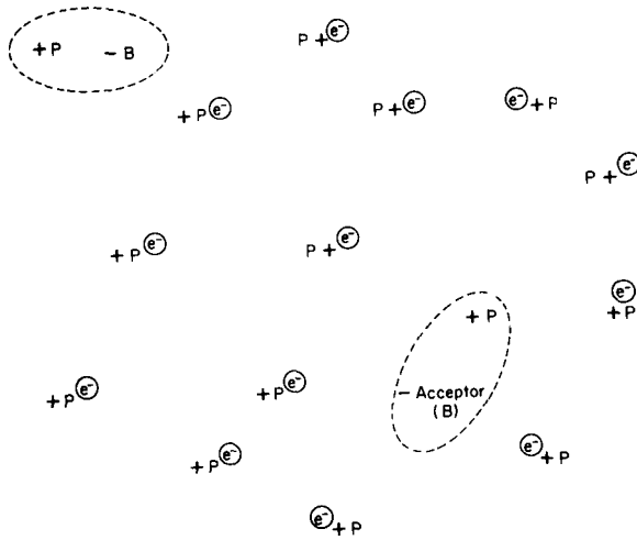
Fig. 12. Hypothetical binding of charged donors to acceptors.
