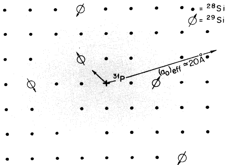
Fig. 9. Donor wave functions in Si and \text{Si}_{29} nuclei: schematic.
