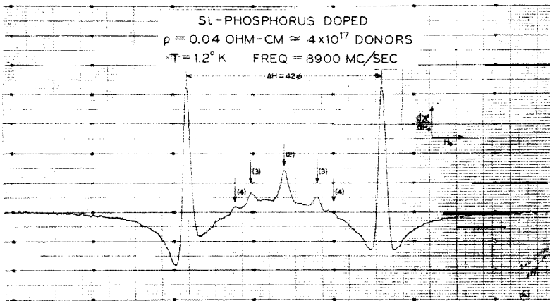
Fig. 10. a) Hyperfine structures of donor EPR at increasing donor (P) concentrations the Mott-Anderson metal-insulator transition. b) Example of well-developed cluster lines.
