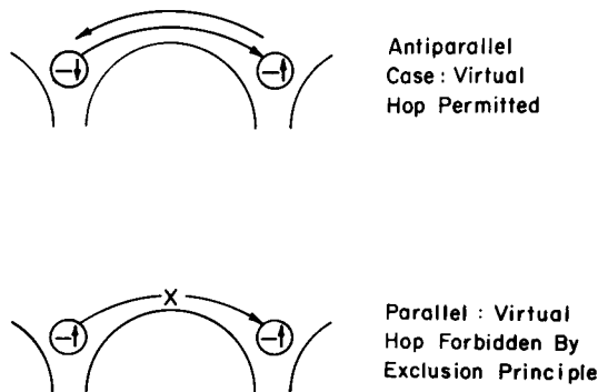
Fig. 2. Virtual hopping as the origin of superexchange.
