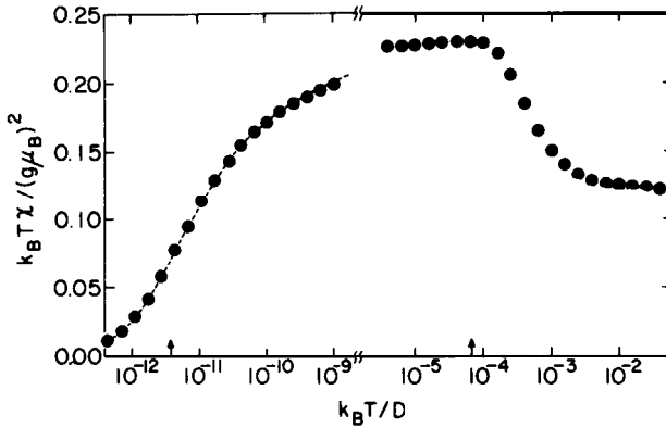
Fig. 8. Susceptibility of the "Anderson Model" showing equivalence to Kondo. (from Krishna-Murthy et al (29))
