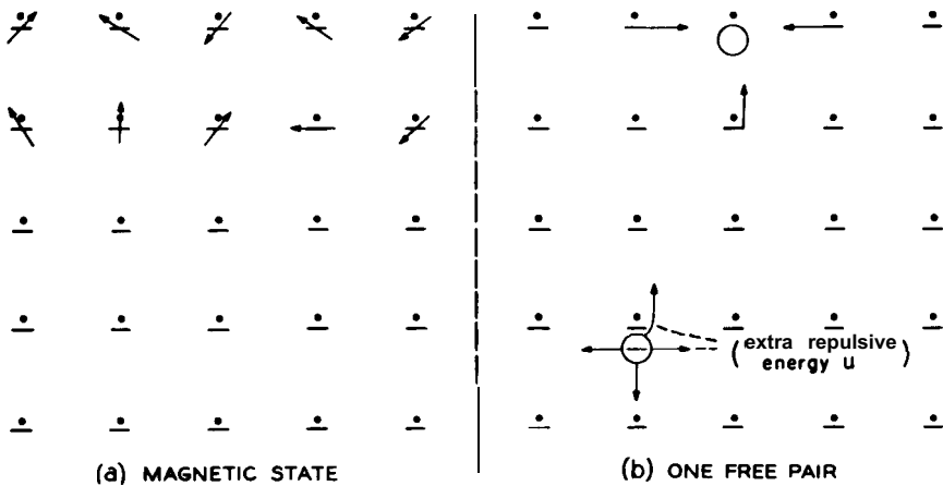
Fig. 1. Mott-Peierls mechanism for magnetic state. State with free pair has extra repulsive energy "U" of two electrons on same site.
