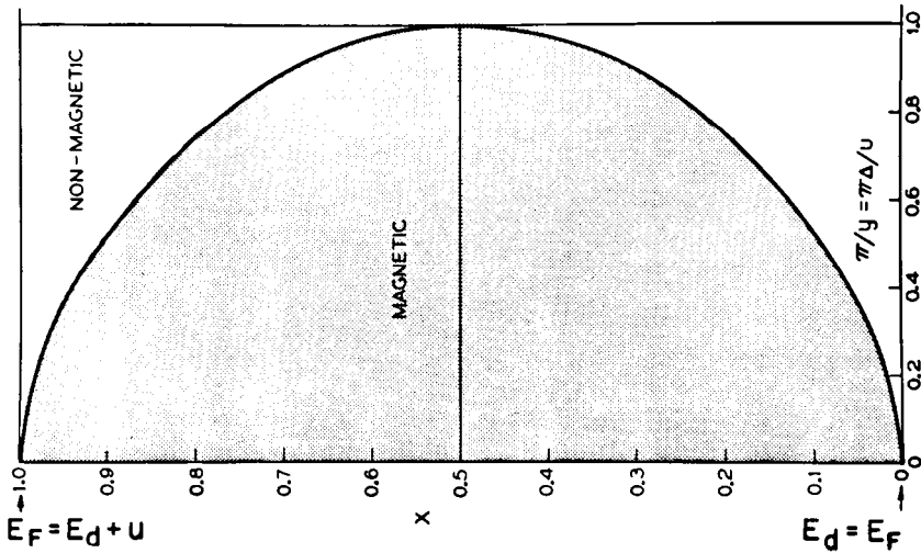
Fig. 6. Magnetic region of parameter space in the "Anderson Model".
