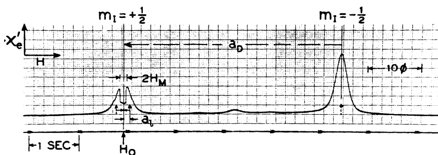
DEMONSTRATION OF THE INHOMOGENEOUS BROADENING IN P-DOPED SILICON ( \rho = 0.25 \Omega \text{ CM} , T = 1.2^\circ \text{ K} , H_0 = 3000 \phi ) IN THE ENDOR TECHNIQUE SPIN PACKETS ARE FLIPPED AS INDICATED BY ARROWS
