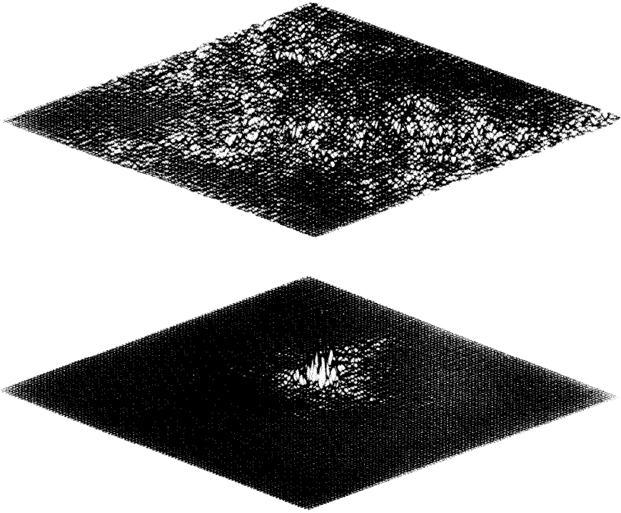
Fig. 18. Computer demonstration of localization (courtesy of Yoshino and Okazaki).
