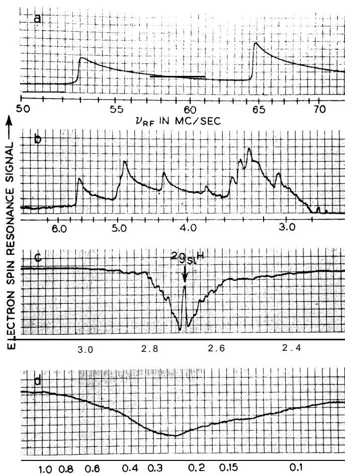
DOUBLE RESONANCE SPECTRUM IN P-DOPED Si. \approx 2 \times 10^{18} \text{ P/CM}^3 , T = 1.3^\circ \text{ K} , \nu_e \approx 9000 \text{ MC/SEC}
