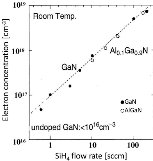
FIGURE 15. Electron concentrations in GaN (●) and AlGaN (○) as a function of SiH 4 flow rate.
