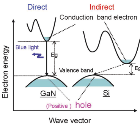
FIGURE 1. Band structures of GaN (direct transition type) and Si (indirect transition type).
