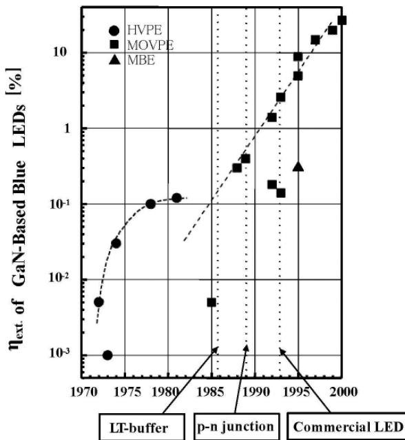
FIGURE 16. Chronological developments in external quantum efficiency, \eta_{ext} of nitride-based blue LEDs (1971–2000).
