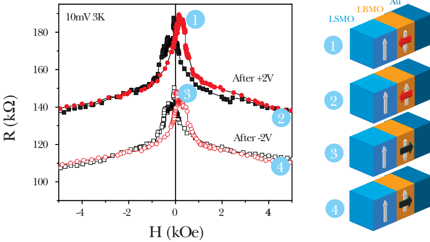
Figure 9. Four state resistance of a tunnel junction composed of a biferroic tunnel barrier ( La_{0.1}Bi_{0.9}MnO_3 ) between a ferromagnetic electrode of La_{2/3}Sr_{1/3}MnO_3 and a nonmagnetic electrode of gold. The states 1-4 correspond to the magnetic (white arrows) and electric (black arrows) polarizations represented on the right of the figure. From Gajek et al. 44 .
