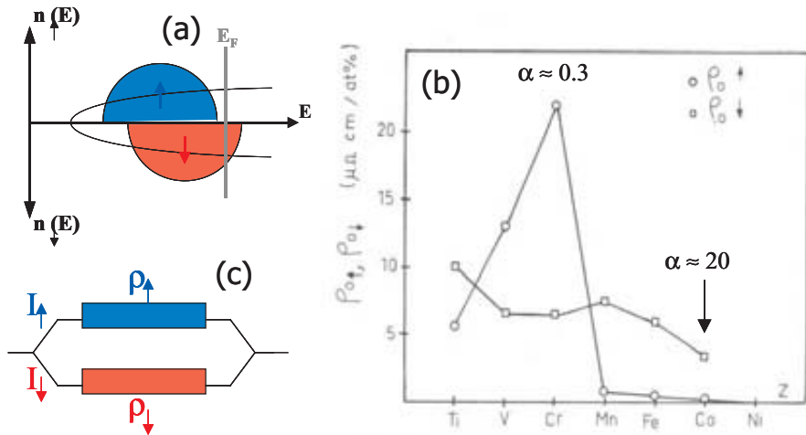
Figure 1. Basics of spintronics. (a) Schematic band structure of a ferromagnetic metal showing the energy band spin-splitting . (b) Resistivities of the spin up and spin down conduction channels for nickel doped with 1% of several types of impurity (measurements at 4.2 K) 4 . The ratio \alpha between the resistivities \rho_{0\downarrow} and \rho_{0\uparrow} of the spin \downarrow and spin \uparrow channels can be as large as 20 (Co impurities) or, as well, smaller than one (Cr or V impurities). (c) Schematic for spin dependent conduction through independent spin \downarrow and spin \uparrow channels in the limit of negligible spin mixing ( \rho_{\uparrow\downarrow} = 0 in the formalism of Ref.[4]).
